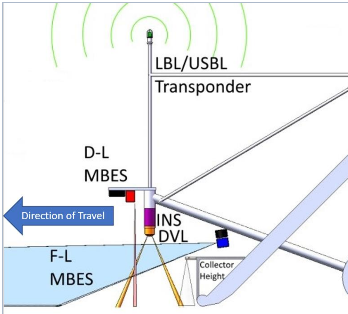
Figure 3-17. PCV navigation system
