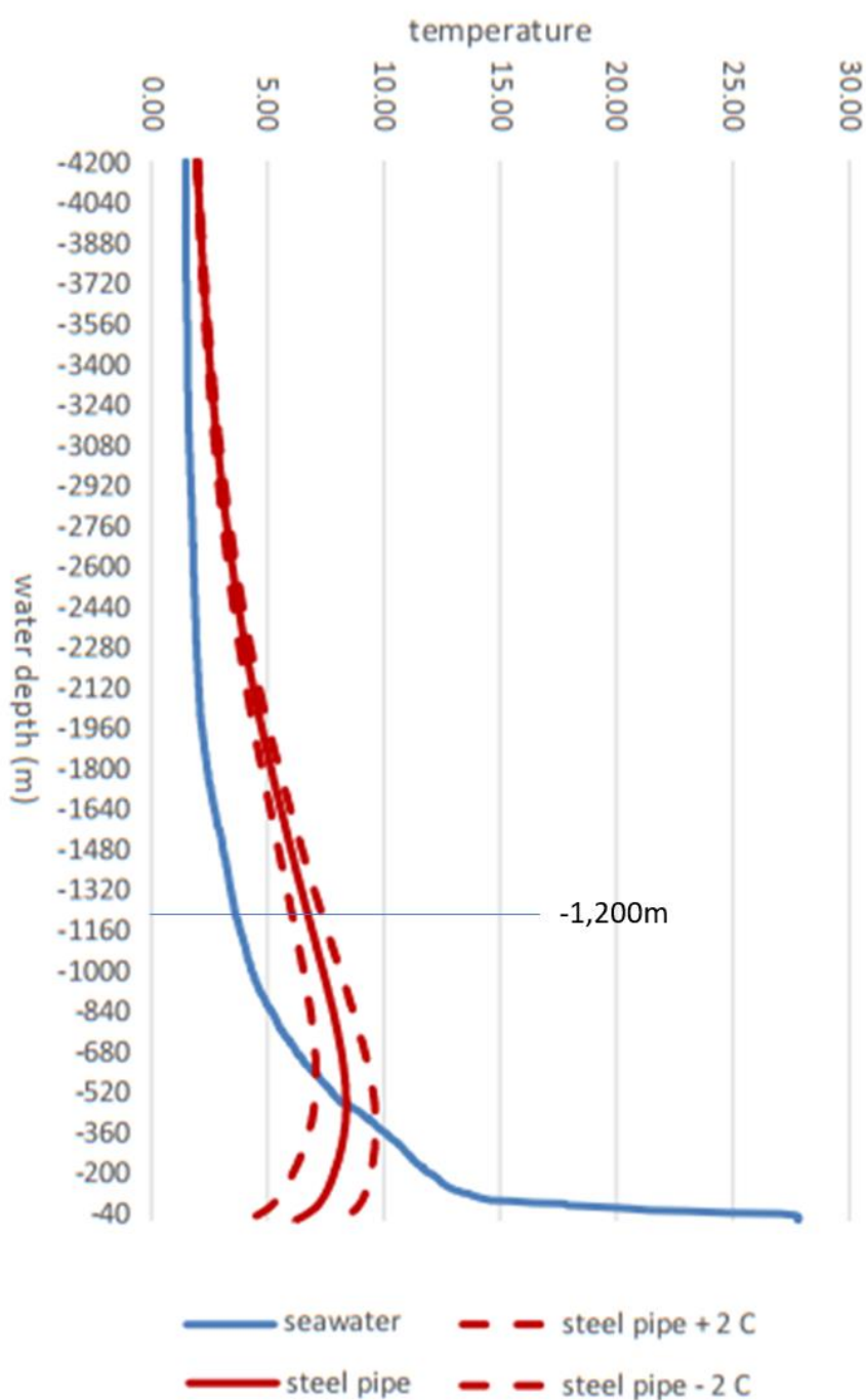
Figure 3-13. Modelled return water temperature and ambient seawater temperature ( ^\circ\text{C} ) at depth (m)
