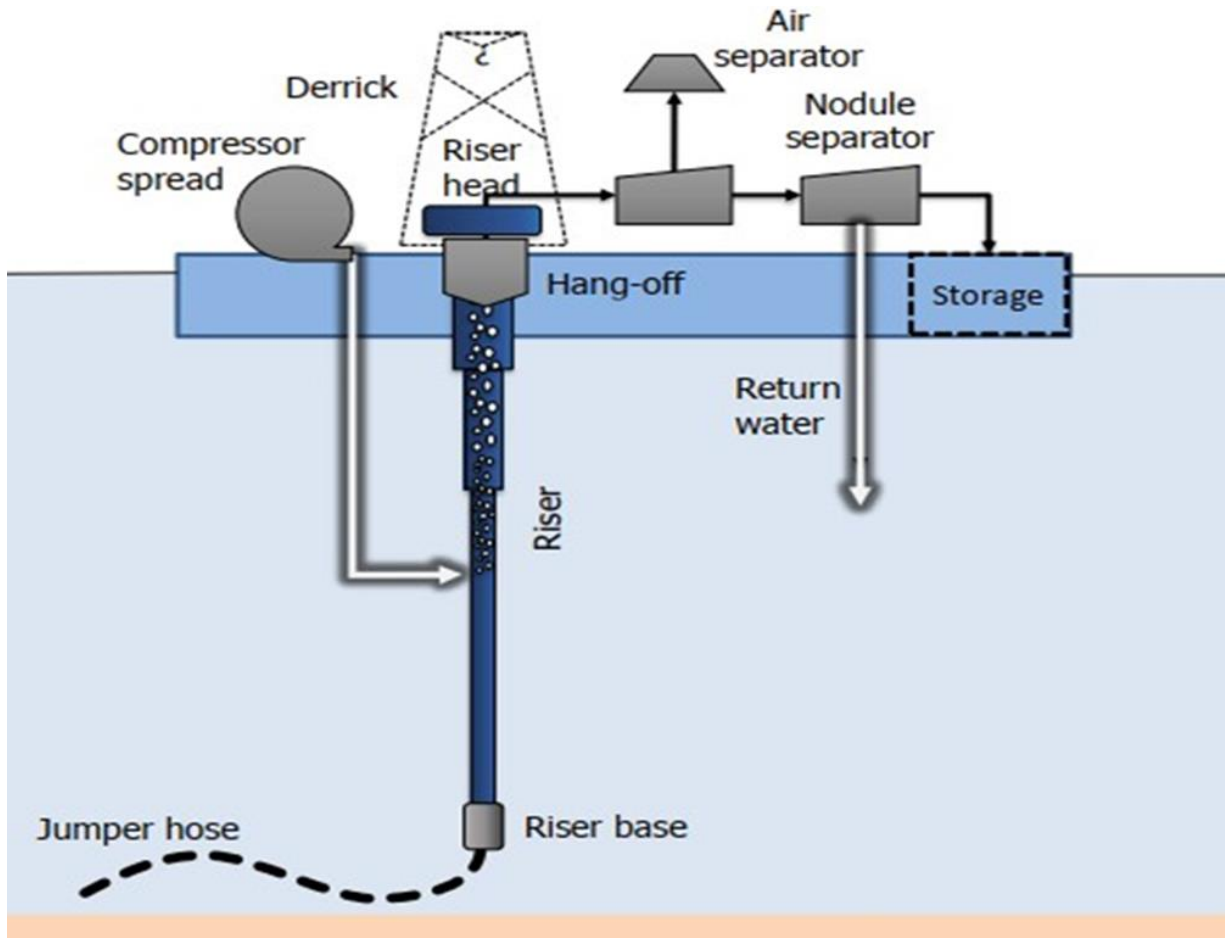
Figure 3-11. Air lift system
