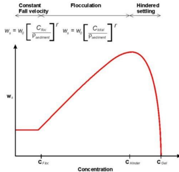
Figure 7-5. Sediment settling velocity model
