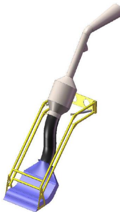
Figure 3-9. Clearance Arms
