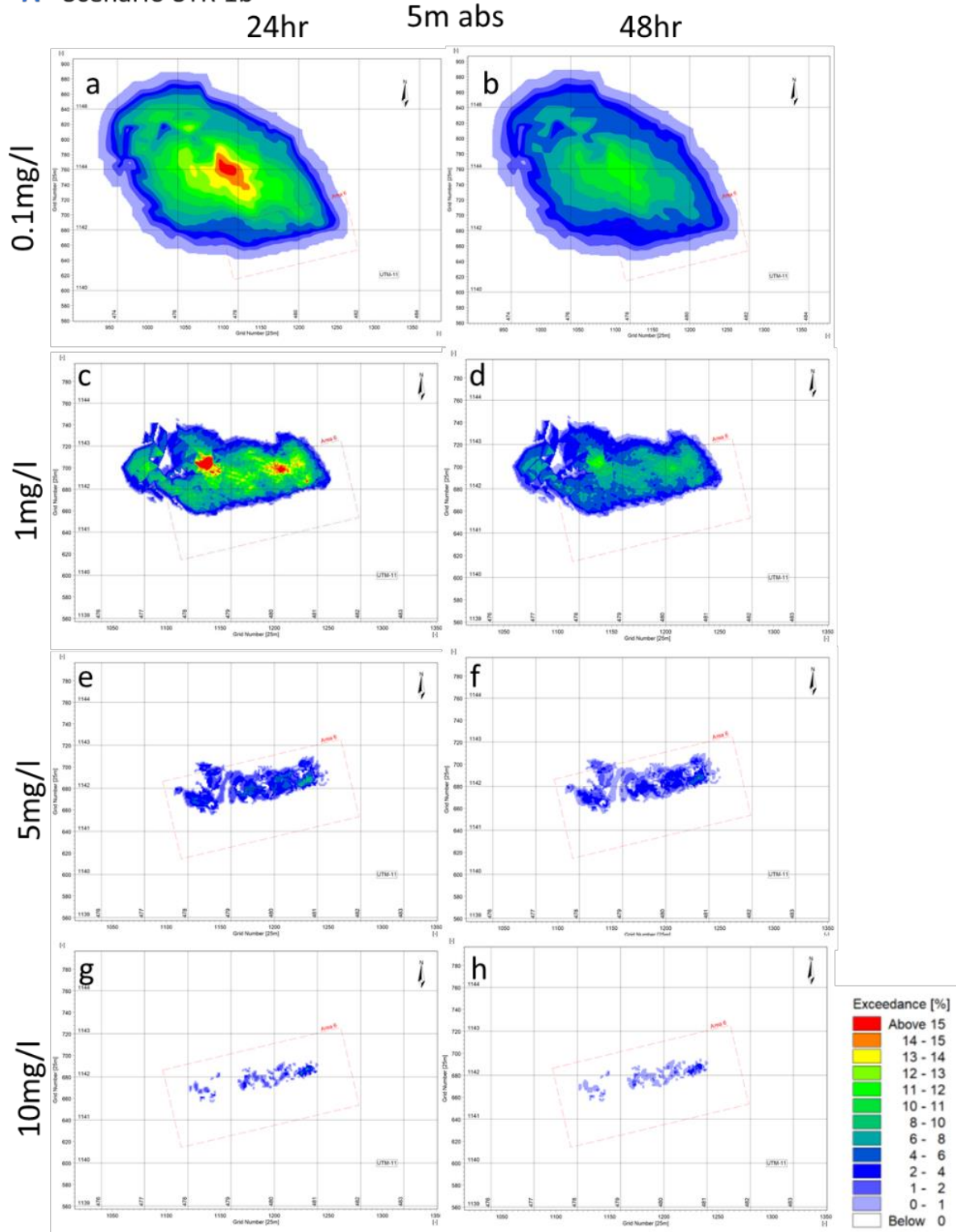
Figure 7-10. Benthic plume scenario model results showing exceedance percentage of 0.1, 1.0, 5.0 and 10.0 mg/l, at 5m and 20m above seabed, from the start of nodule production to 24 and 48 hours post-nodule production for all scenarios.
