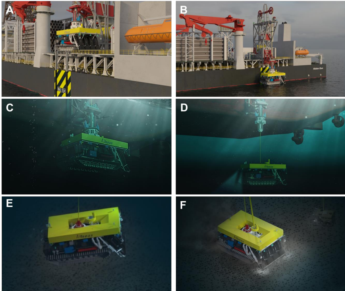
Figure 3-19. PCV deployment and recovery sequence
