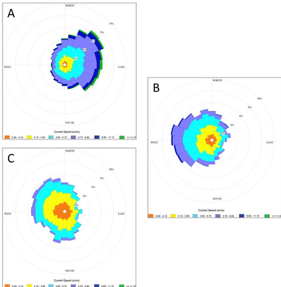
Figure 5-7. Current roses at 498 m (A), 1,232 m (B) and 4,321 m (C)
