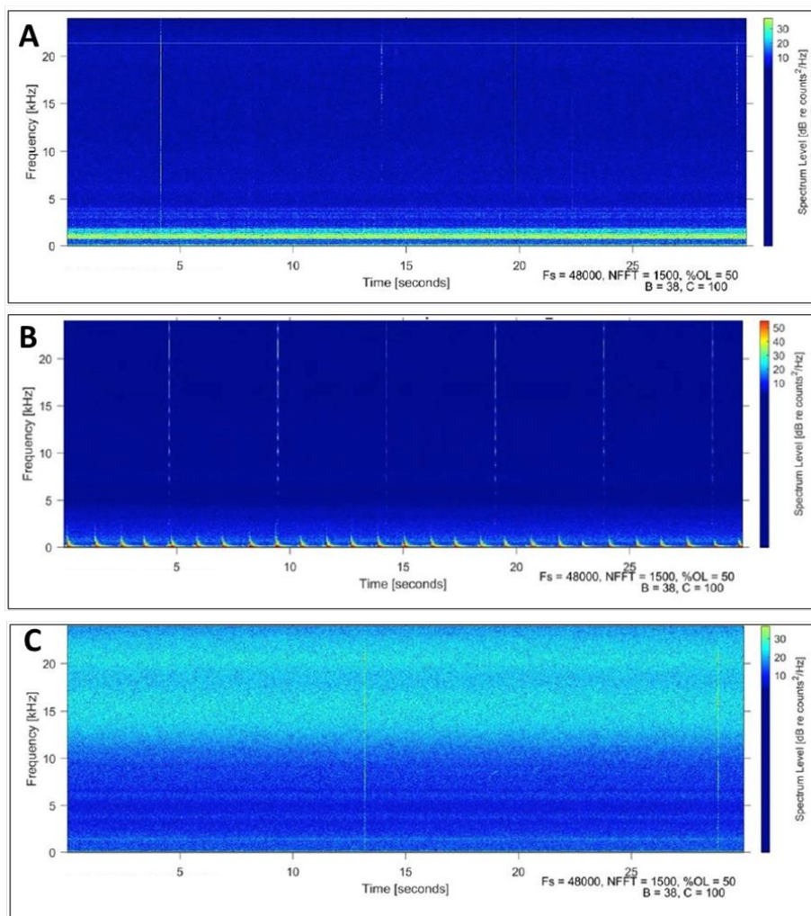
Figure 5-4. Spectrograms from 538 m showing traces for sounds produced by passing vessels (A); geological exploration (B) and weather (C)
