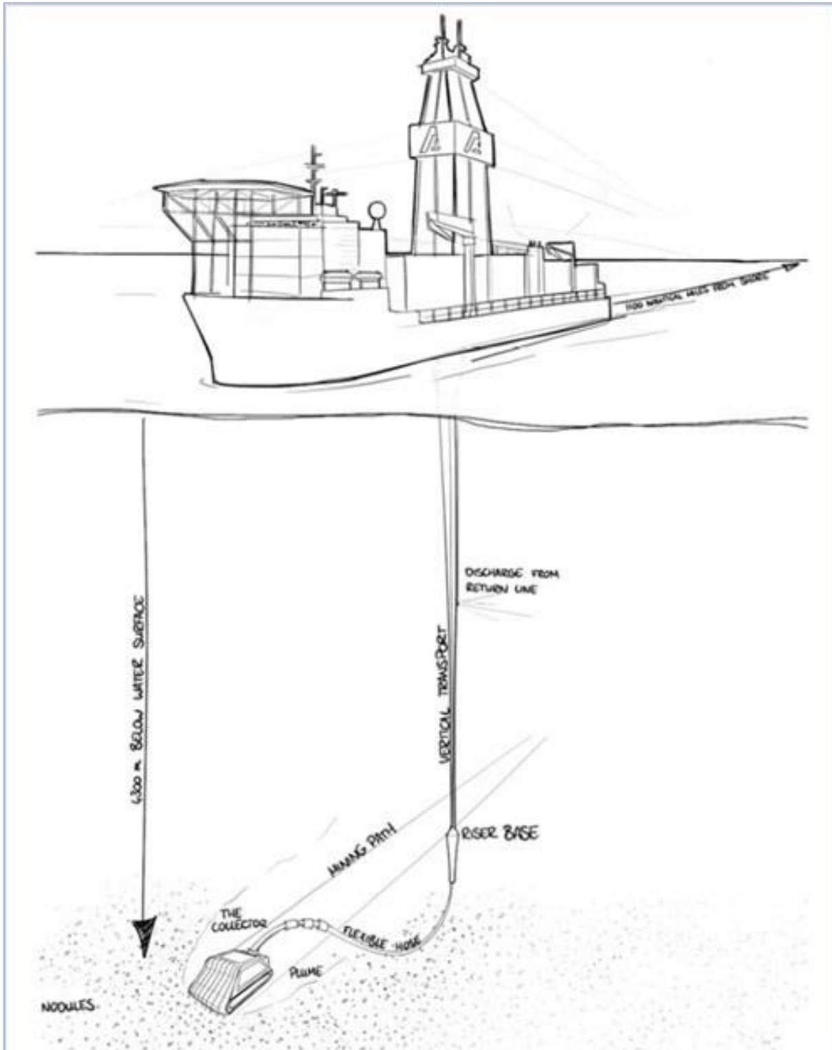
Figure 3-4. Nodule Collection System
