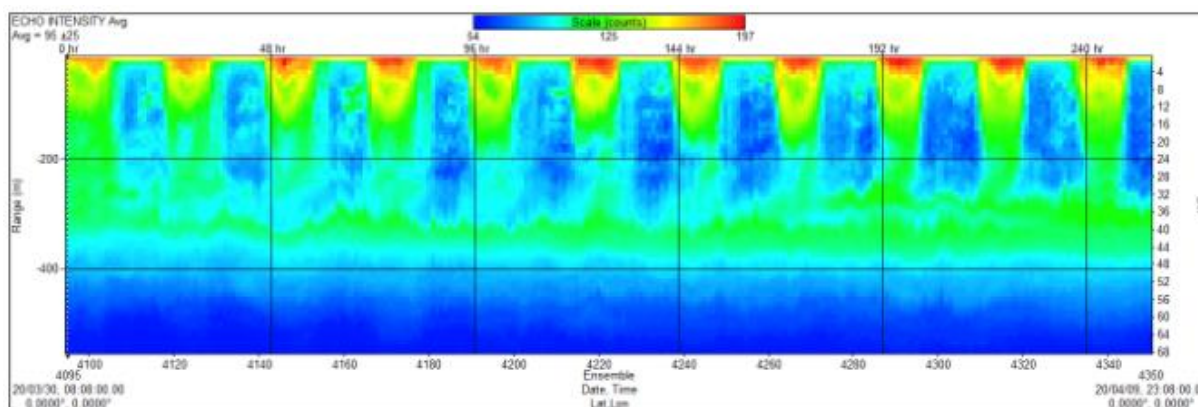
Figure 6-16. Downward looking ADCP backscatter intensity plots (75 kHz) at 500 m depth from March 30 to April 09, 2020
