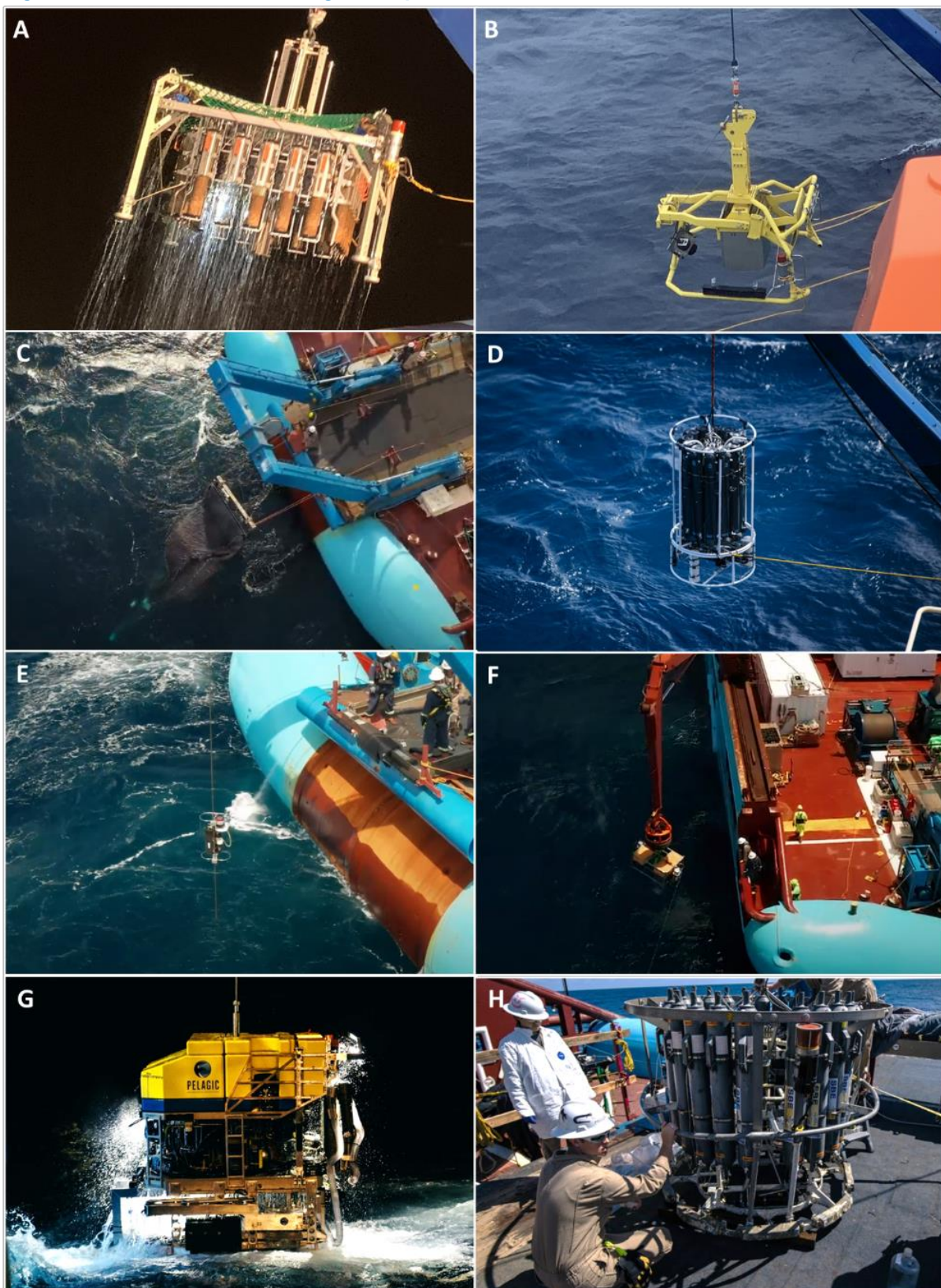
A – Multicore; B – Box-core; C – MOCNESS net; D – Trace metal rosette; E – McLane pump; F – Zooplankton Lander; G – Remotely Operated Vehicle; H – Rosette Sampler
