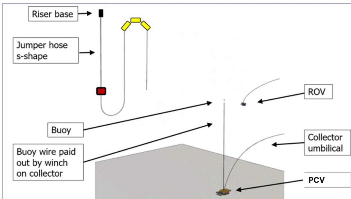
Figure 3-22. Connection configuration
