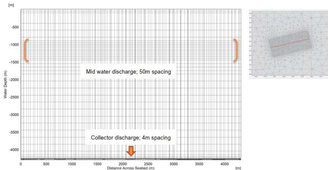
Figure 7-4. Longitudinal slice through test field site*
