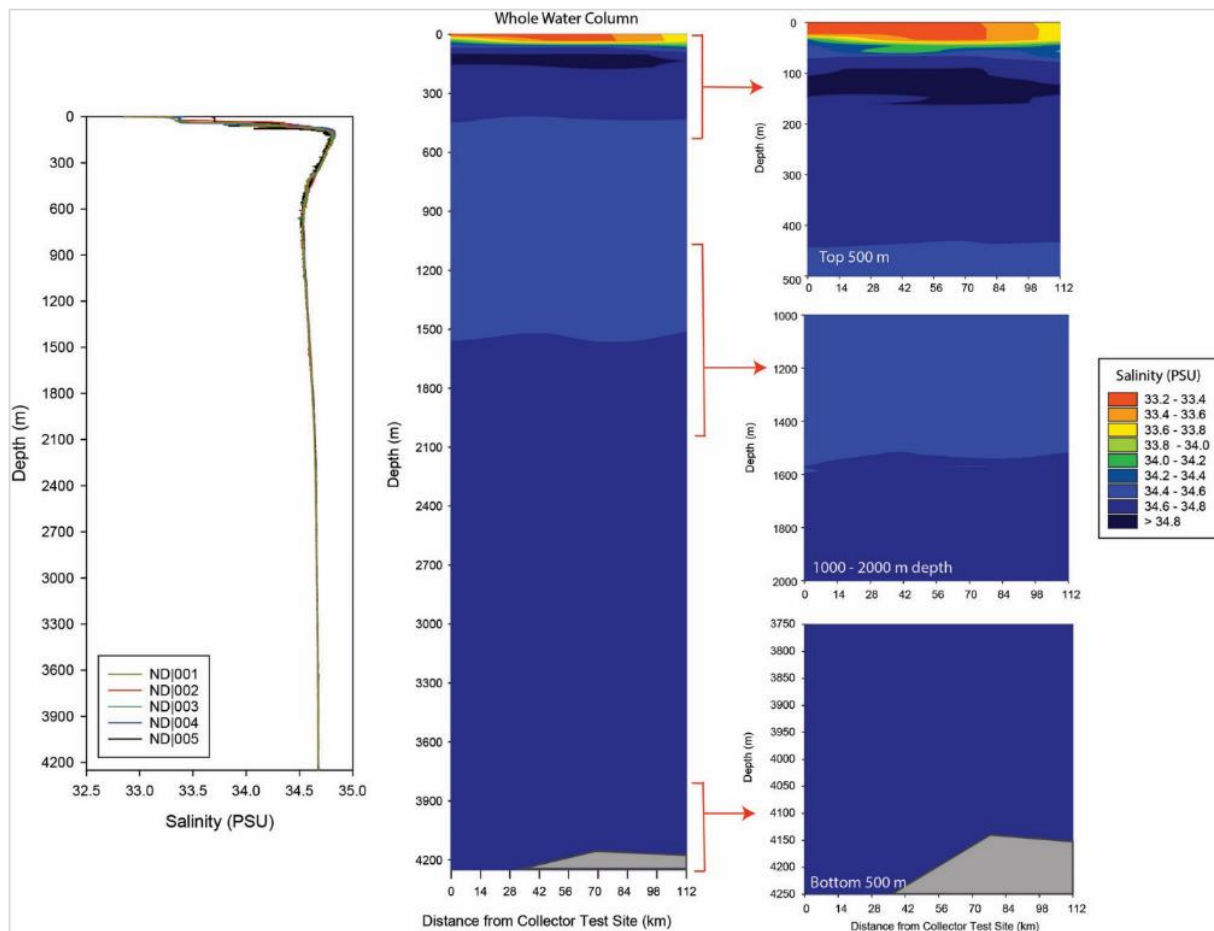
Figure 5-11. Salinity profiles in NORI-D October, 2019
