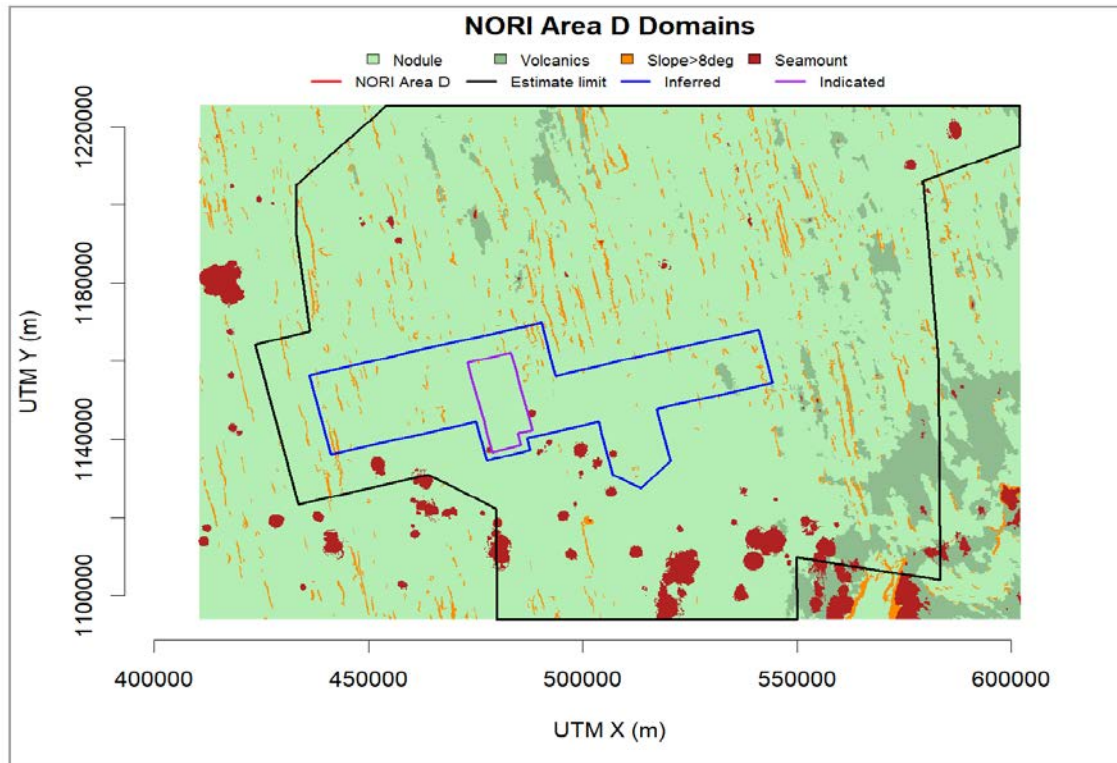
Figure 5-32. NORI-D geological domains
