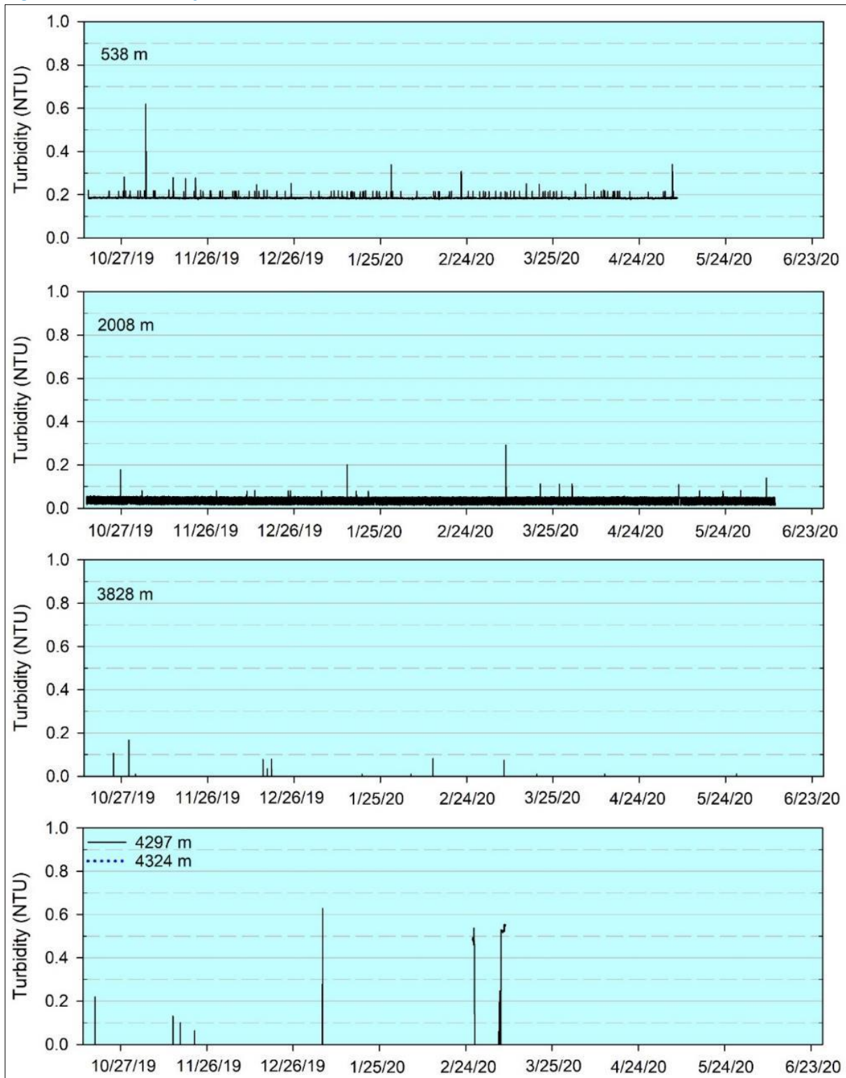
Figure 5-17. Turbidity time series in NORI-D, June 2020
