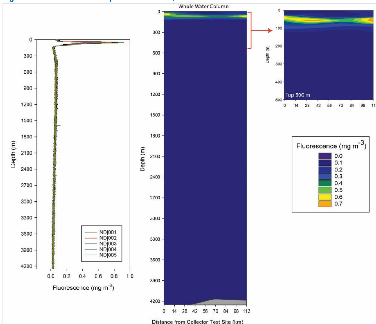
Figure 5-20. Fluorescence profile in NORI-D, October 2019
