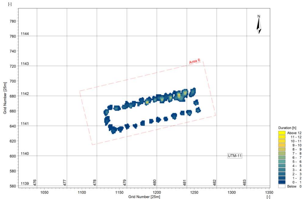
Figure 7-16. Total duration (hours) where 0.1mg/l is exceeded at 50 m below the mid water column discharge point.
