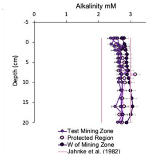
Figure 5-28. Campaign 5A alkalinity results †
