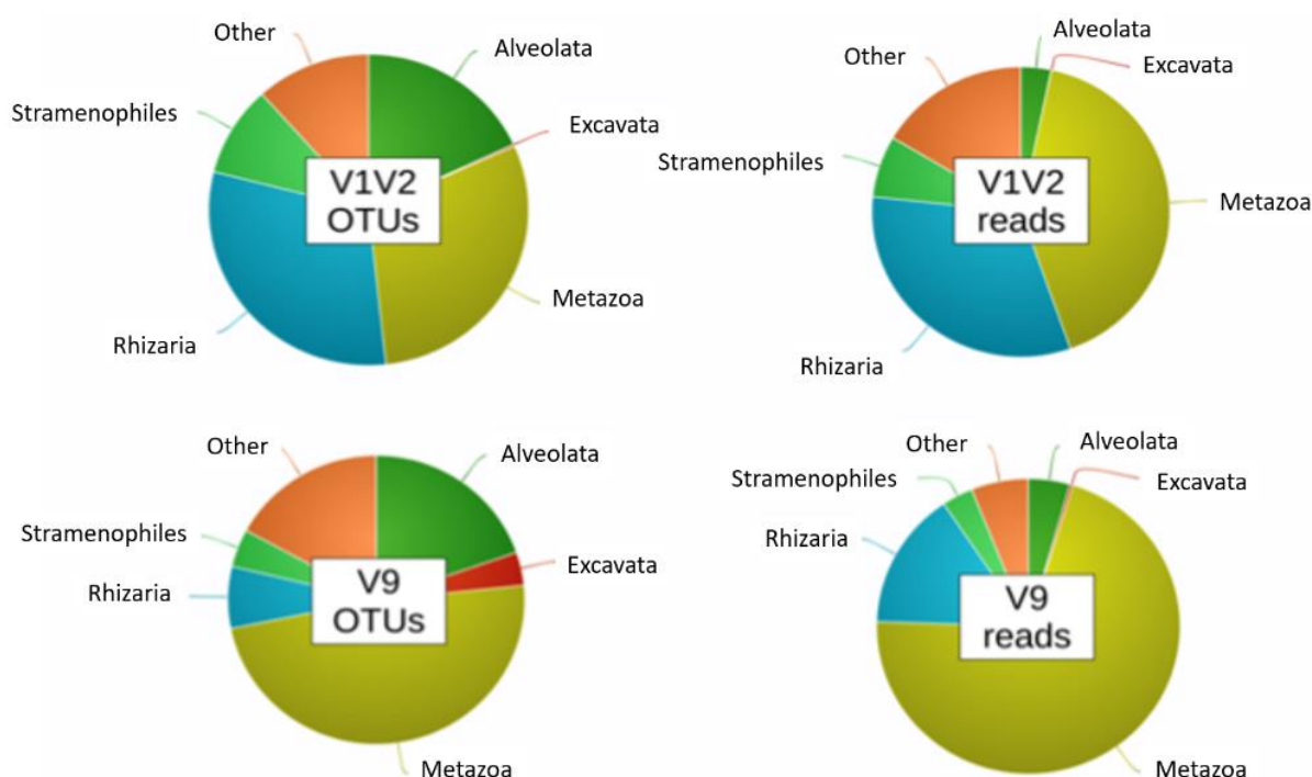
Figure 6-11. Taxonomic composition of eukaryotic communities using V1V2 and V9 markers and considering the richness (number of OTUs) or the abundance (number of reads).
