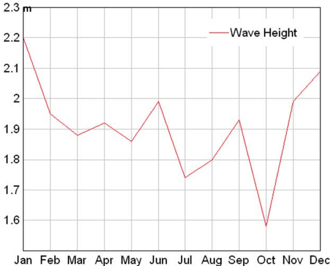
Figure 5-5. Average monthly wave heights in the CCZ
