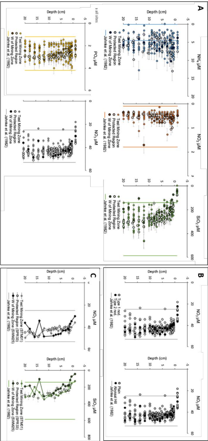
Figure 5-29. Campaign 5A nutrient results
