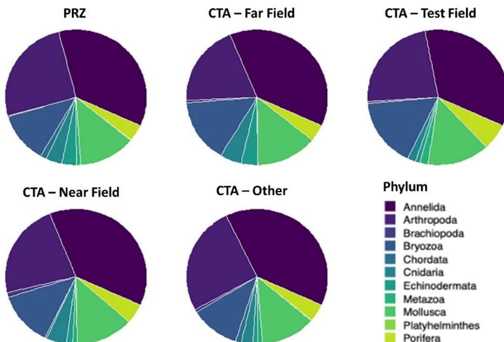
Figure 6-8. Relative abundance of the macrofauna from the NORI-D 5A sites.
