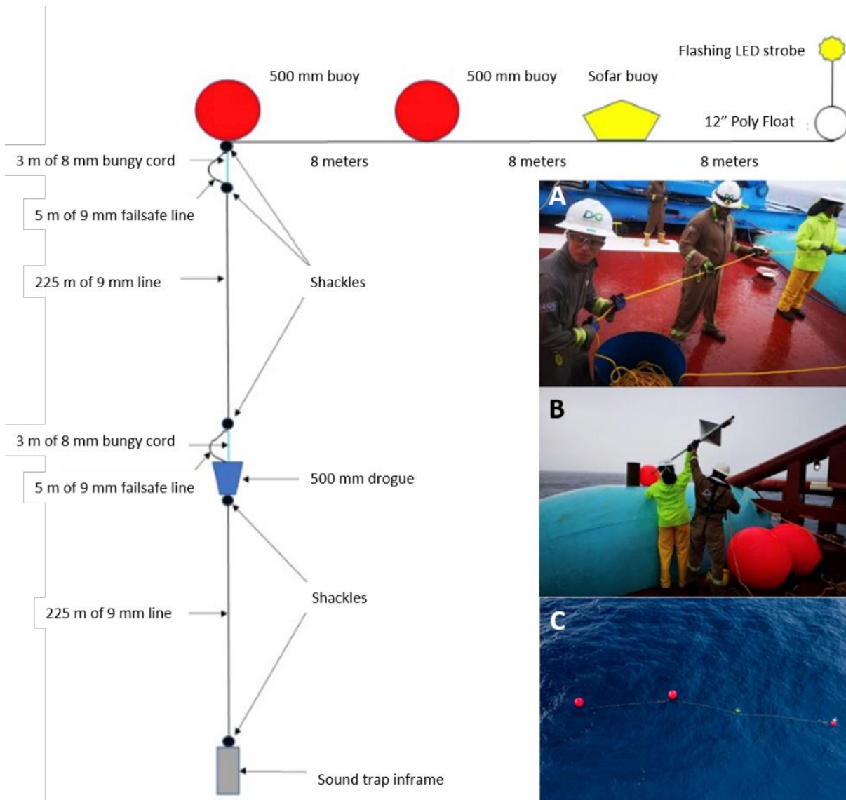
Figure 6-18. Hydrophone setup and operation
