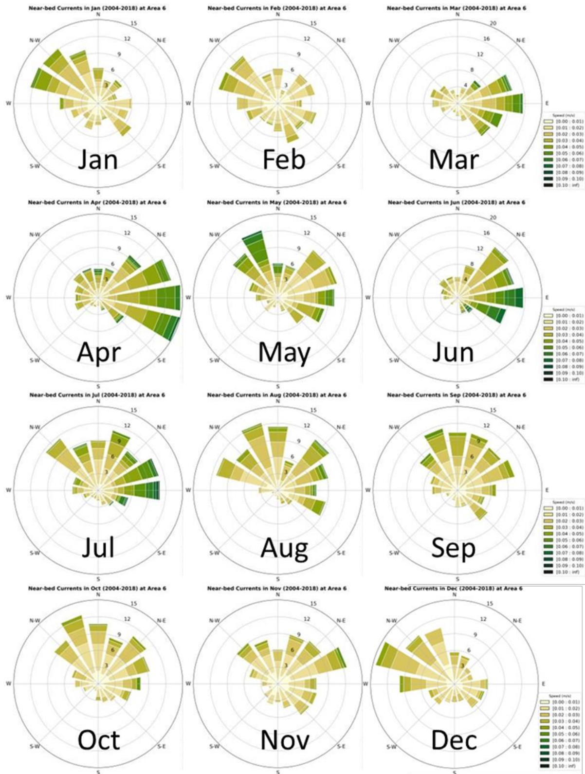
Figure 7-7. Seasonal variability in near bed current conditions (current flowing to) at the location of the long mooring in the NORI-D area based on HYCOM data 2004 to 2018 (HYCOM 2021)
