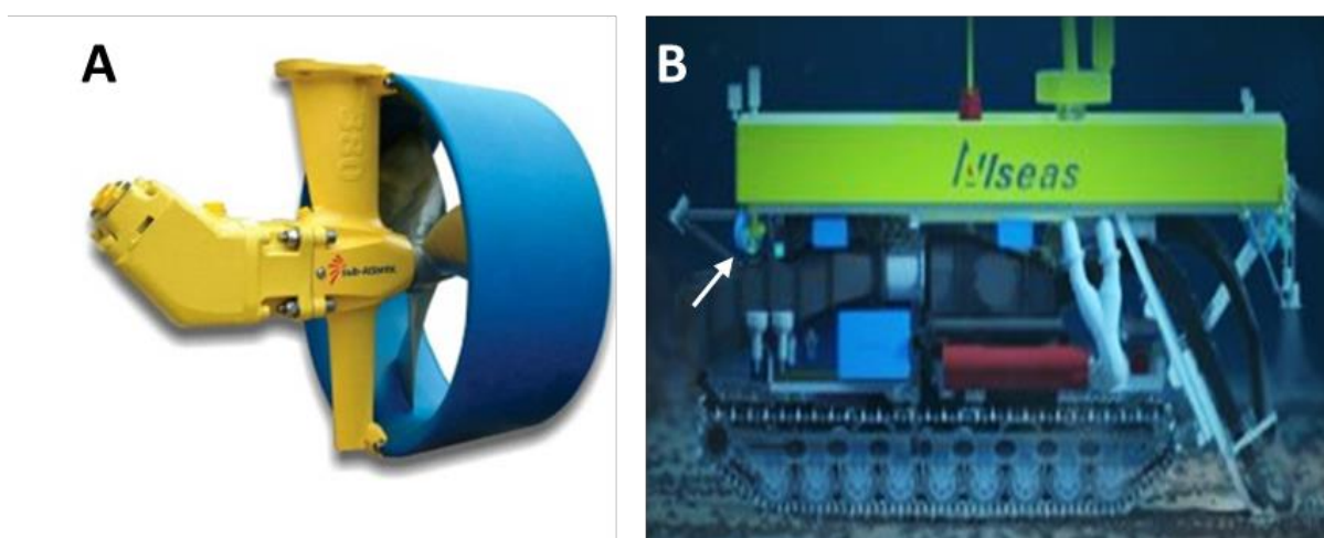
Figure 3-15. Thruster unit (A) and position on the PCV (B - dotted red circles)
