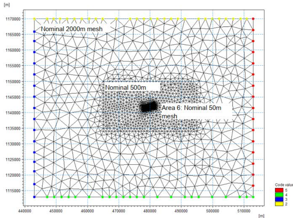
Figure 7-3. Collector test model mesh
