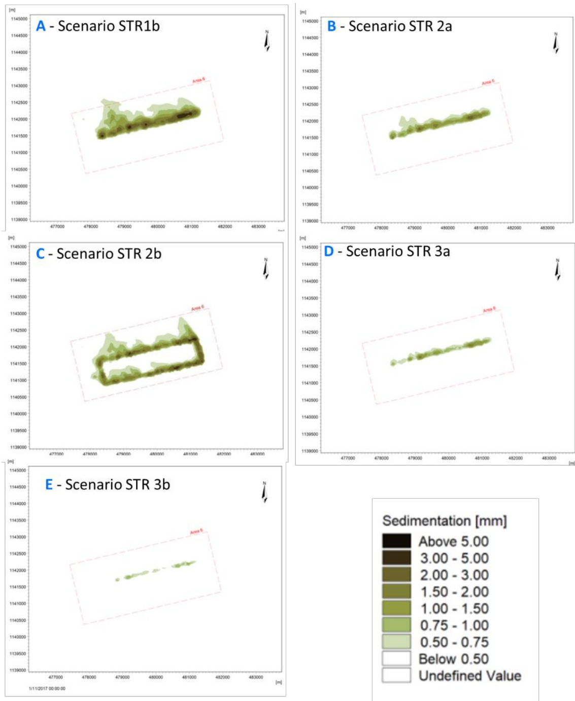
Figure 7-9. Sediment deposition footprints†
