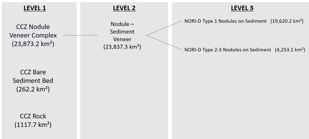
Figure 5-41. Substrate structure of NORI-D
