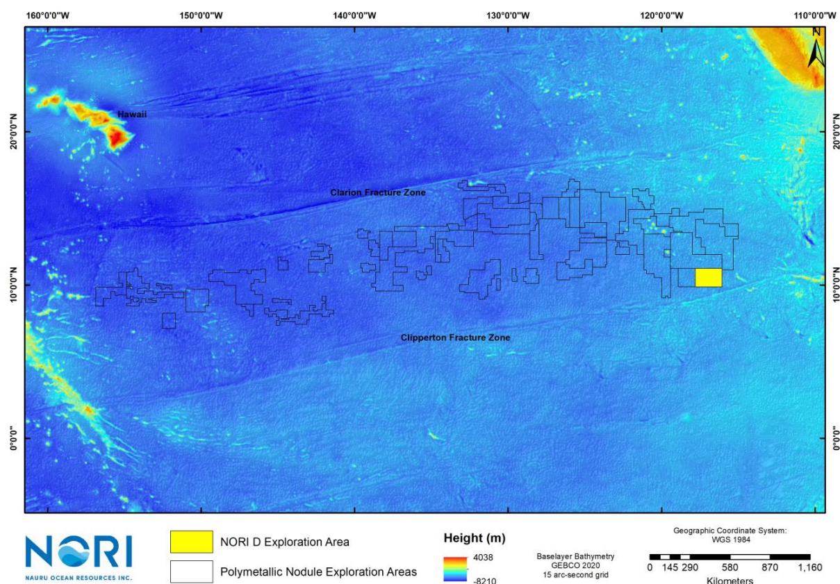
Figure 5-30. Bathymetric overview of the CCZ
