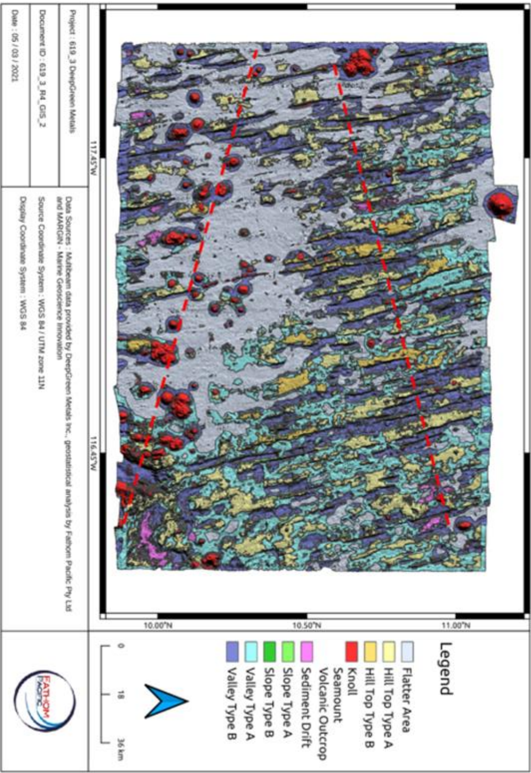
Figure 5-40. NORI-D Level 3 geoforms. Red lines indicate alignment of two knoll-seamount chains.
