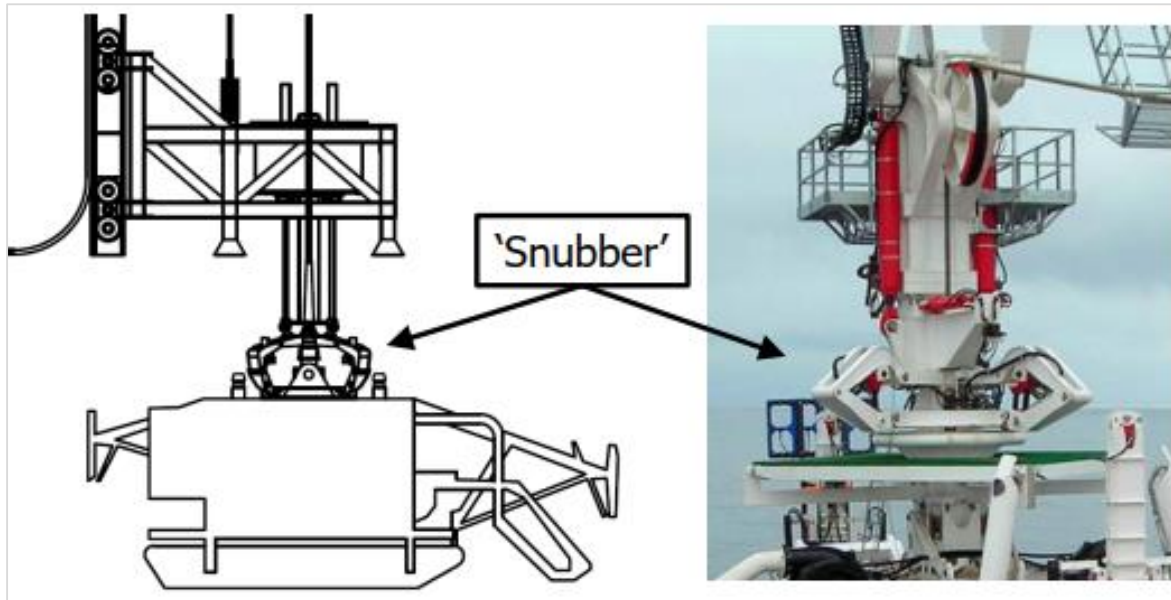
Figure 3-18. Snubber configuration
