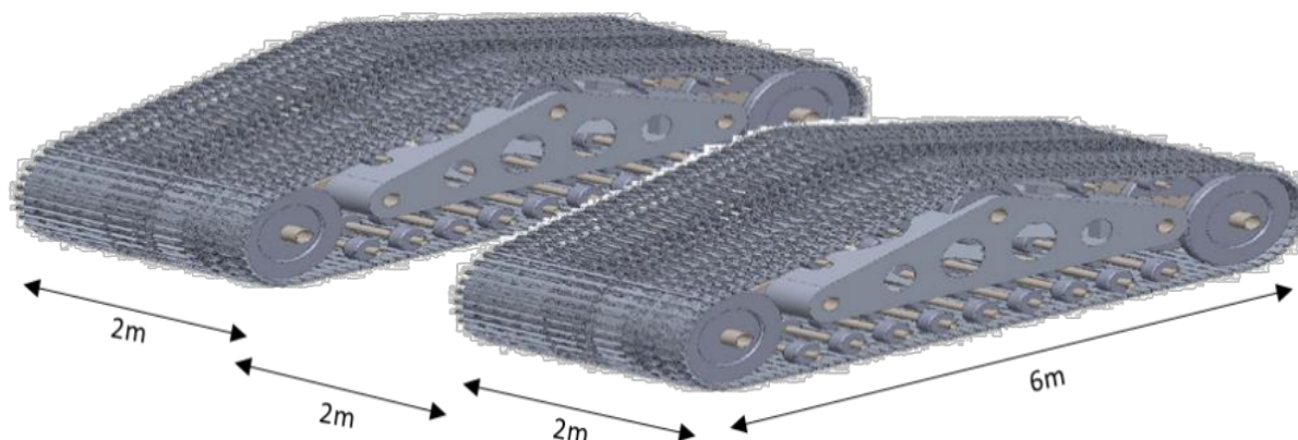
Figure 3-14. PCV track system (A); 2 m wide, 6m apart (B); 6 m long at the base (C)
