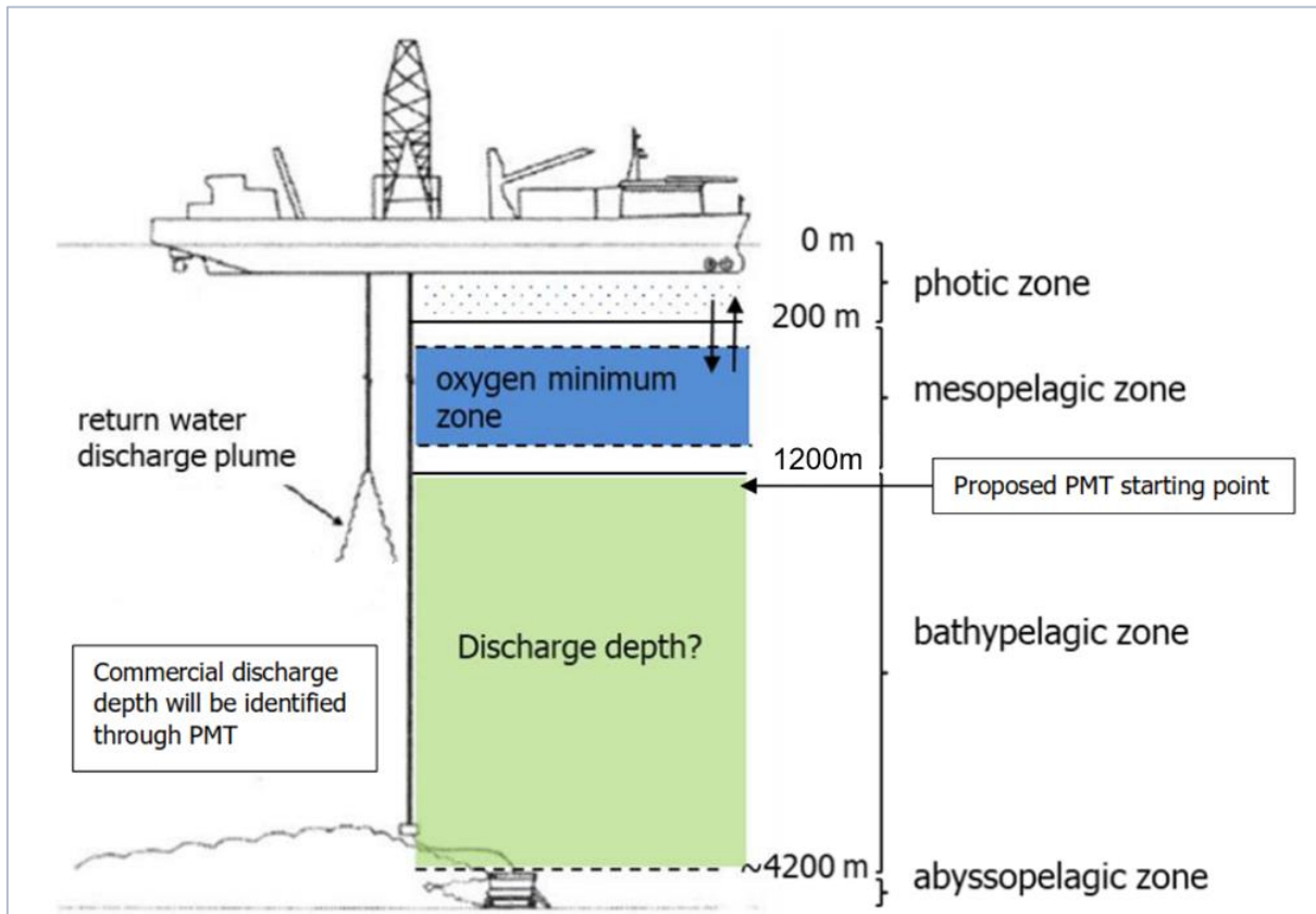
Figure 3-12. Proposed discharge depth for integrated system tests.
