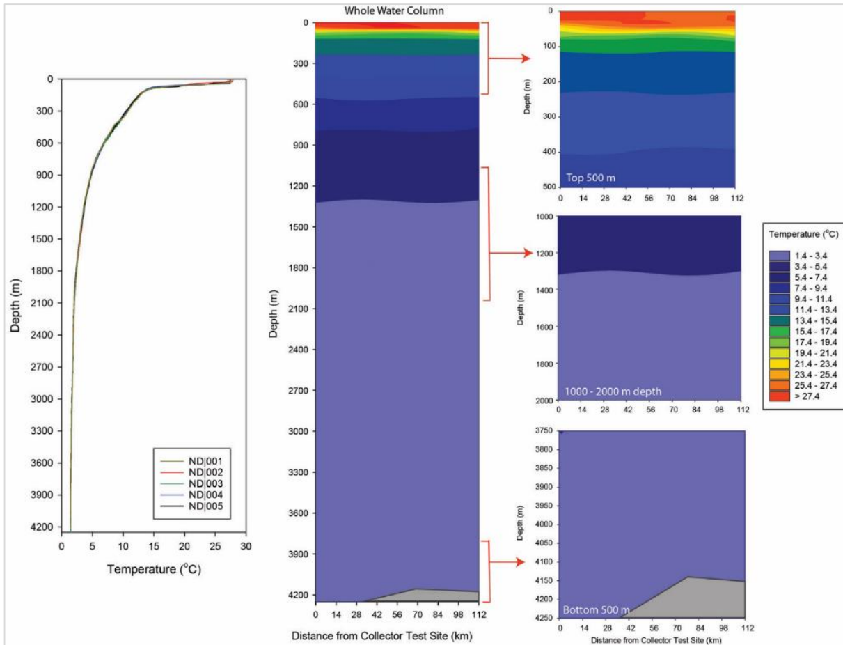
Figure 5-9. In-situ temperature profiles in NORI-D, October 2019
