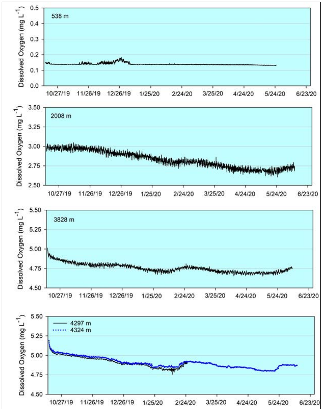
Figure 5-14. Dissolved oxygen time series in NORI-D
