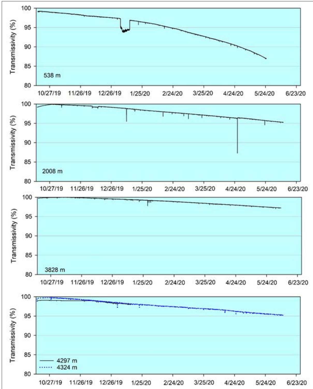
Figure 5-19. Seasonal transmissivity profiles in NORI-D, (Oct, 2019 – Jun, 2020)
