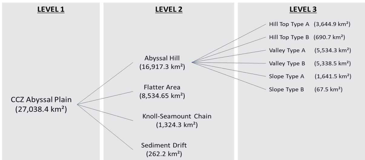
Figure 5-37. Geoform structure of NORI-D
