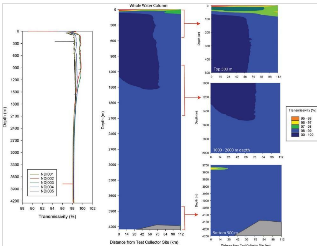
Figure 5-18. Static transmissivity profiles in NORI-D (June 2020)
