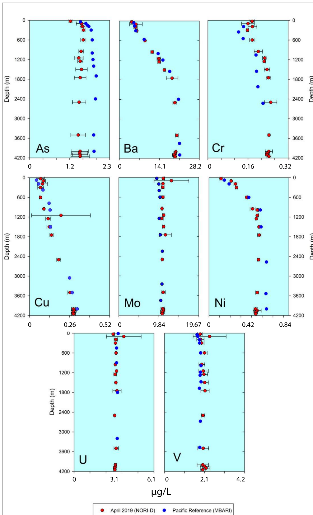
Figure 5-8. Average ( \pm standard deviation) metal and metalloid concentrations by depth
