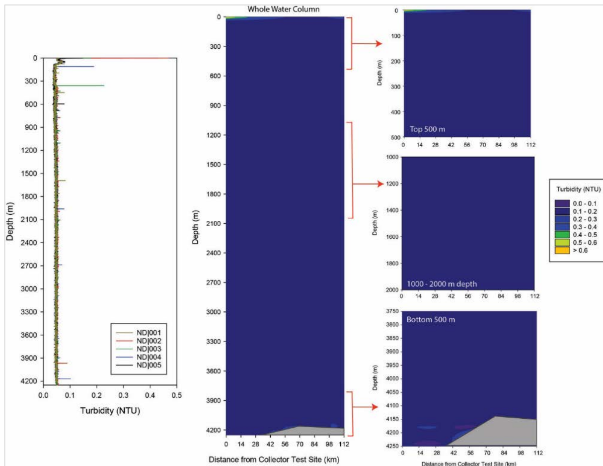
Figure 5-16. Turbidity profiles in NORI-D, October 2019
