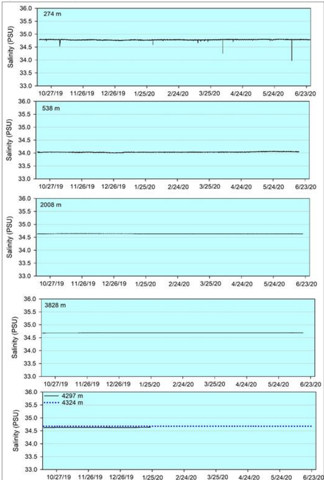
Figure 5-12. Salinity time series in NORI-D
