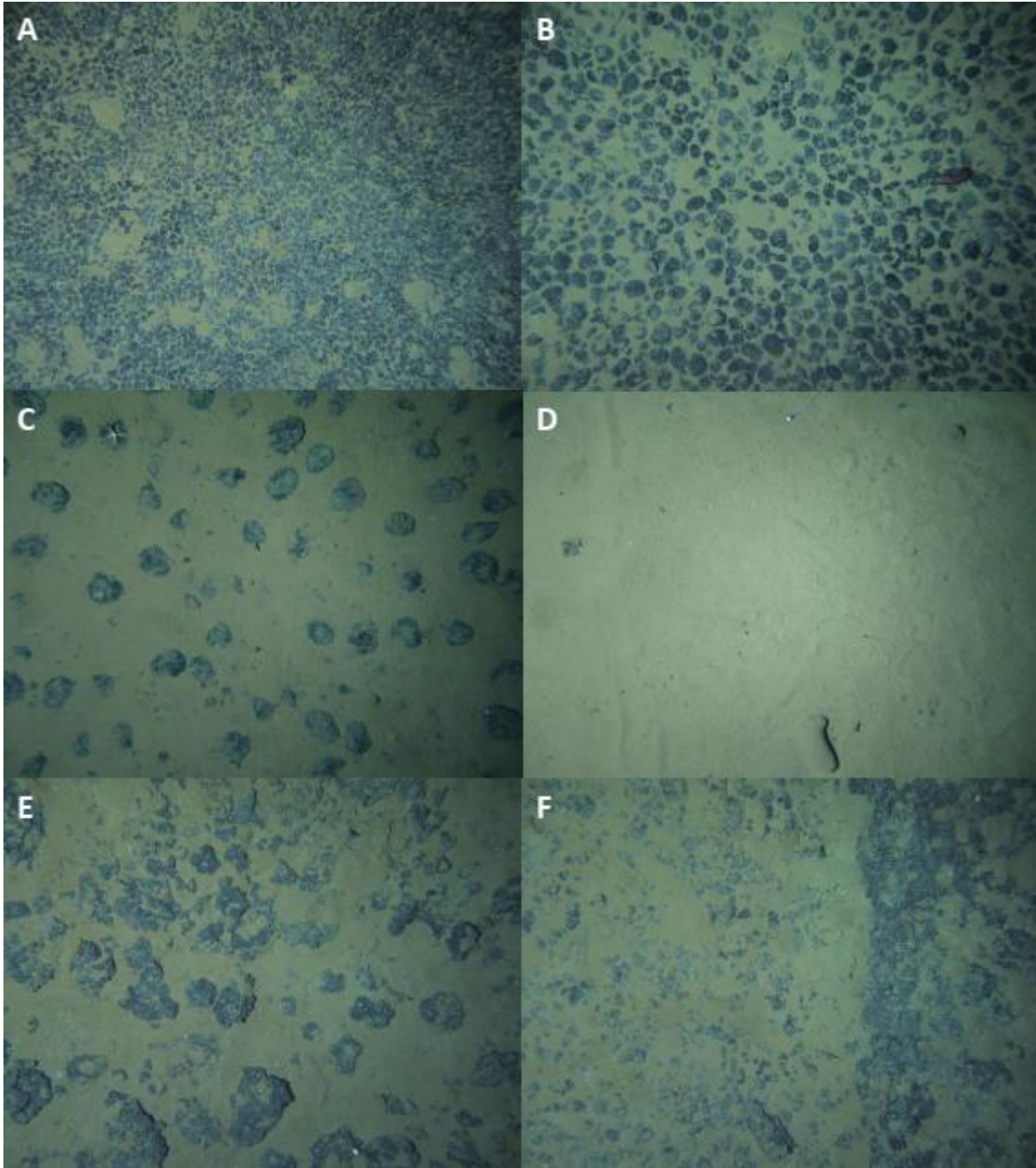
A) Nodules: Type I. B) Nodules: Type II. C) Nodules: Type III. D) Nodule-free. E and F: Exposed rock: E) Fragments; F) Bedrock
