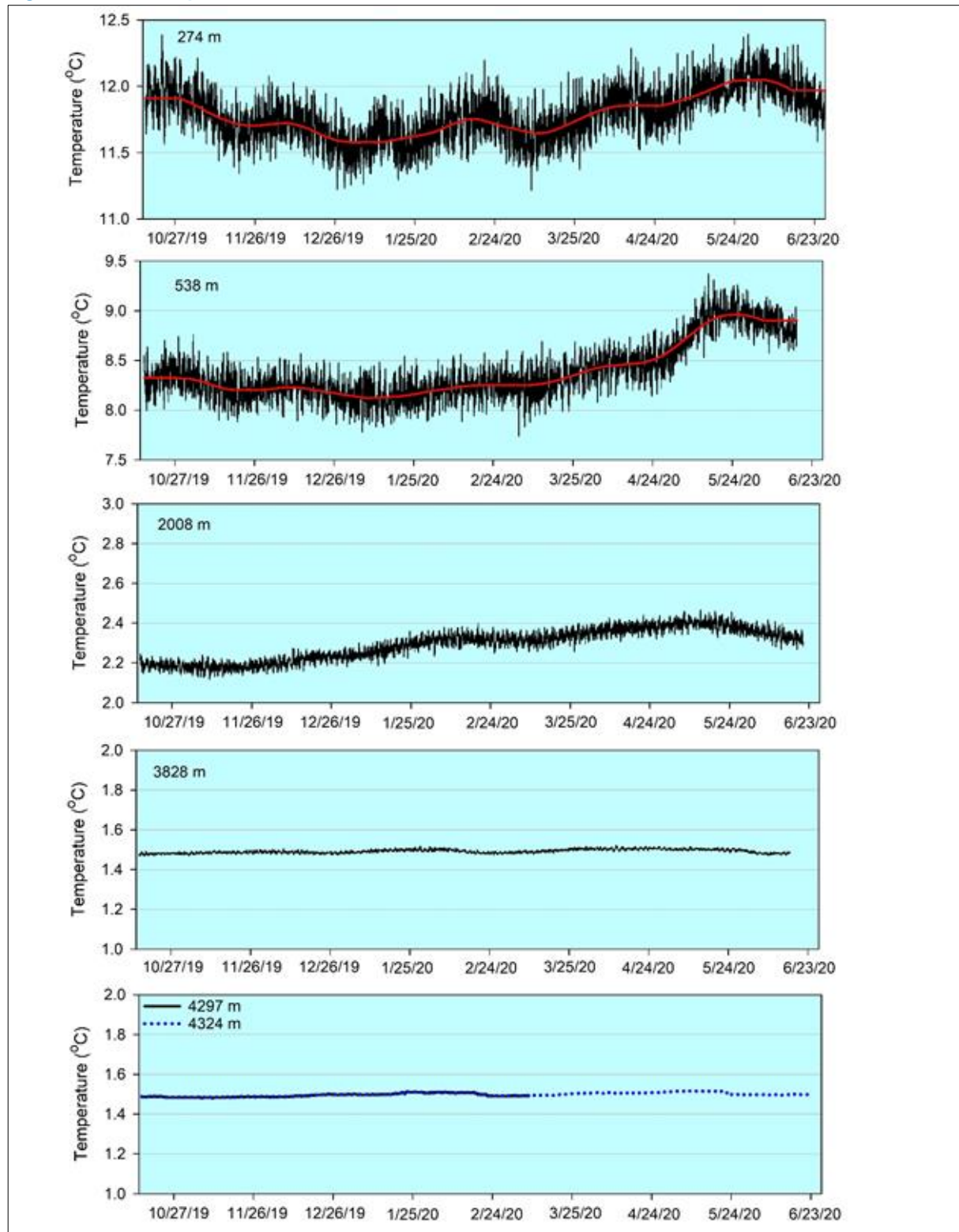
Figure 5-10. Temperature time series in NORI-D
