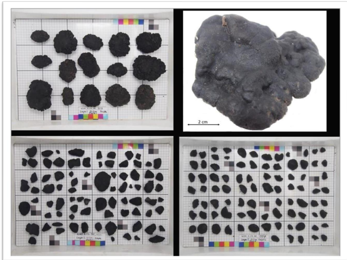
Figure 5-34. NORI-D nodule collection showing ranges of sizes.
