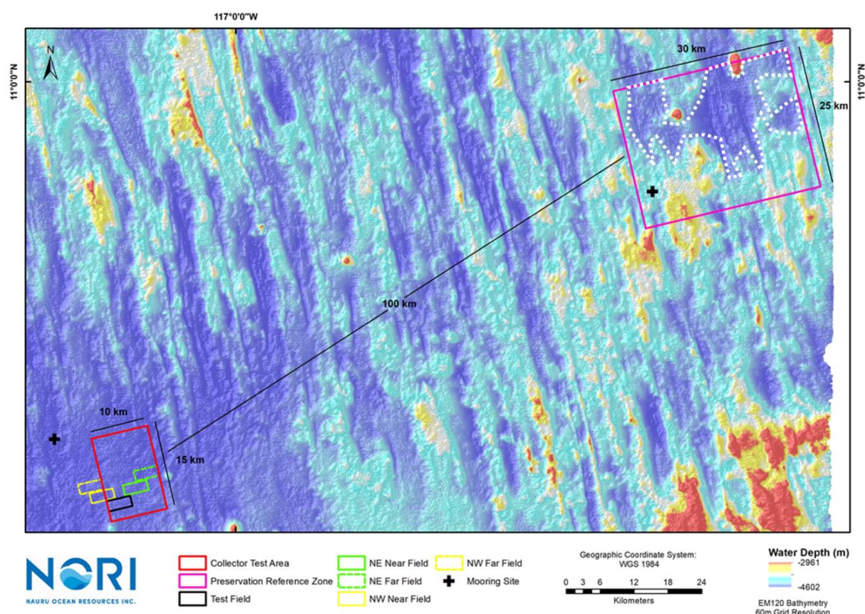
Figure 3-3. Bathymetric map of NORI-D showing relative locations of the CTA and PRZ
