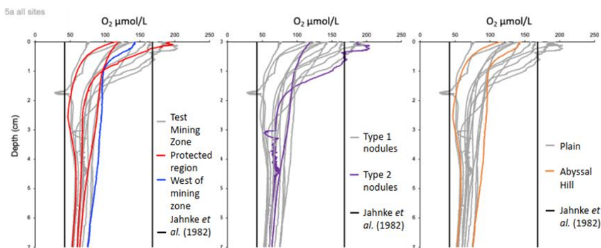
Figure 5-27. Campaign 5A ex-situ oxygen results †‡
