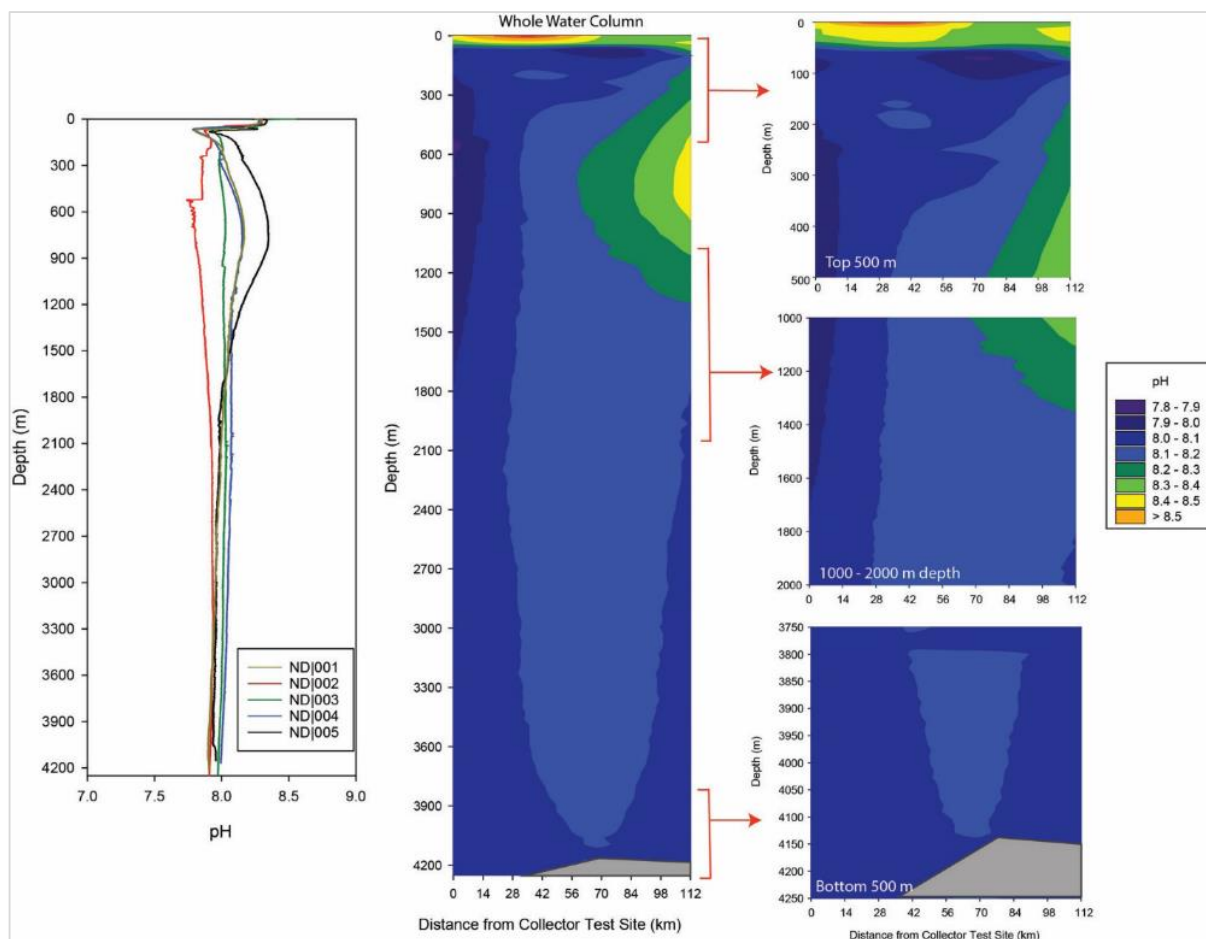
Figure 5-15. pH profiles in NORI-D, October 2019
