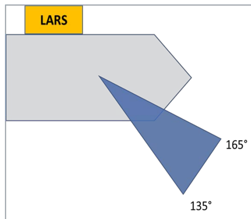
Figure 3-20. Design to provide wave shielding during lowering through the splash zone
