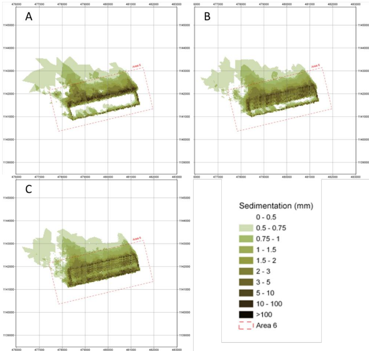
Figure 7-13. Cumulative sedimentation for base case (A), Shift 1 (B) and Shift 2 (C)
