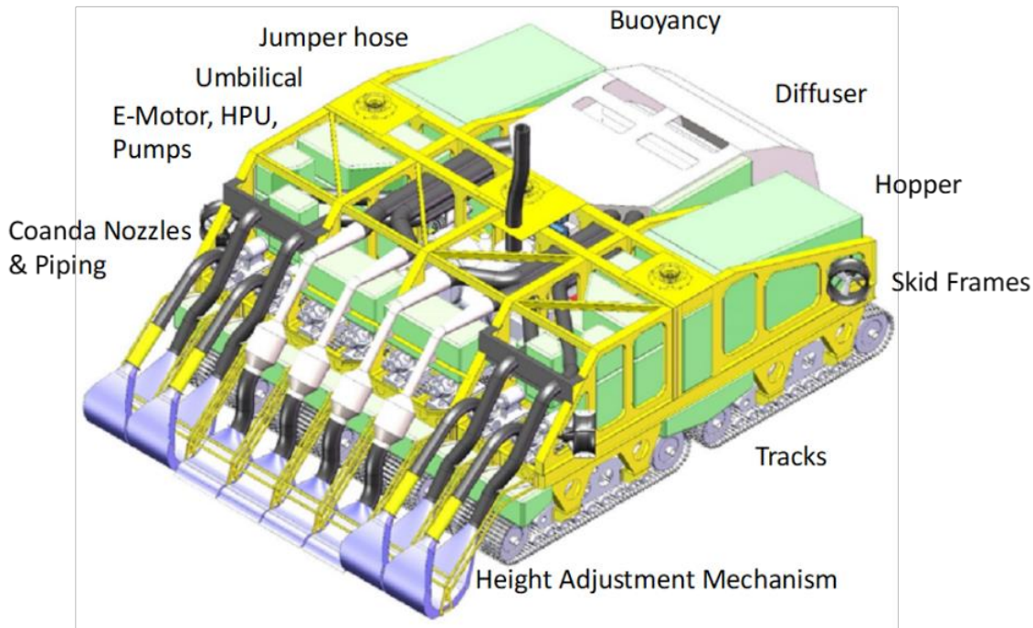
Figure 3-7 Main components of the Prototype Collector Vehicle
