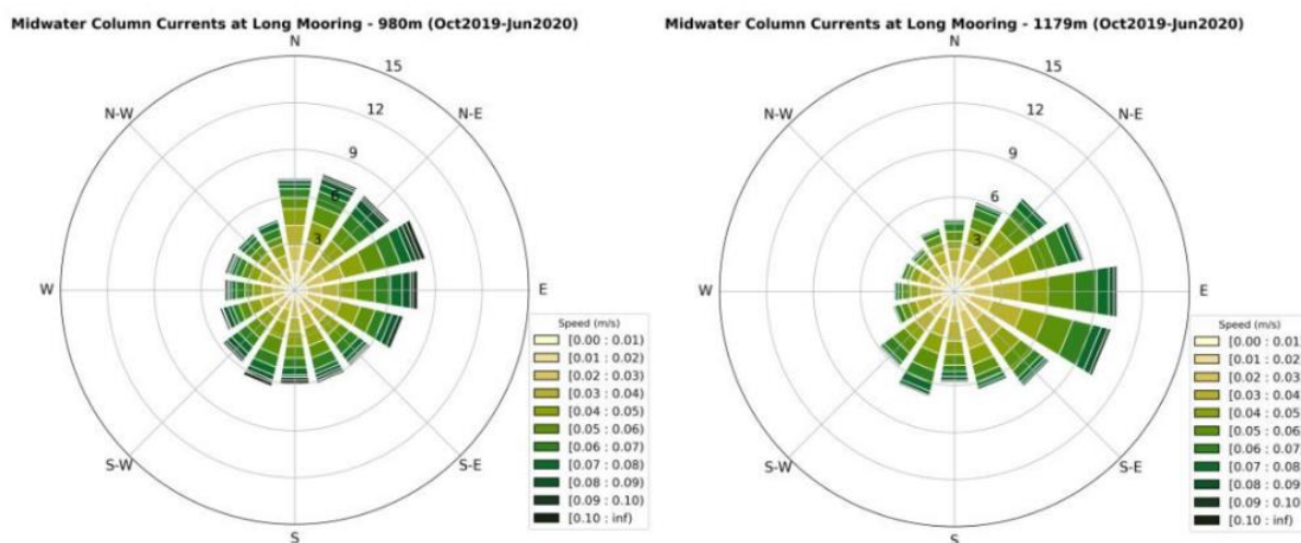
Figure 7-6. Measured current conditions at the NORI-D long mooring (current flowing to) at approximately 980m and 1179m (right) below the surface - 14 October 2019 to 26 June 2020
