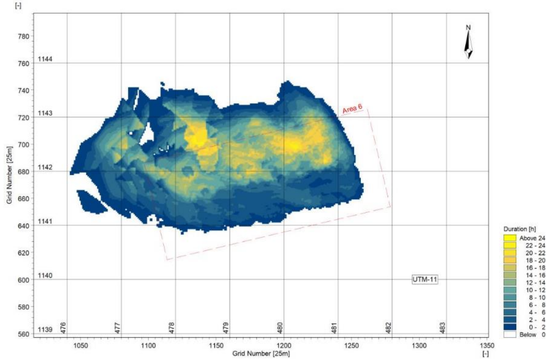
Figure 7-14. Total duration (hours) where 1mg/l is exceeded at 5 m above the seabed.
