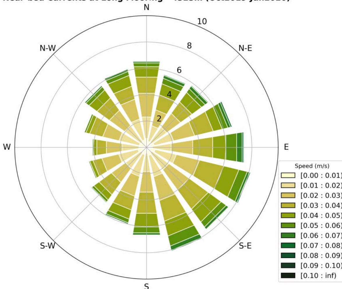
Figure 7-2. Summary of measured near bed current data from NORI-D (14 October 2019 to 26 June 2020)
