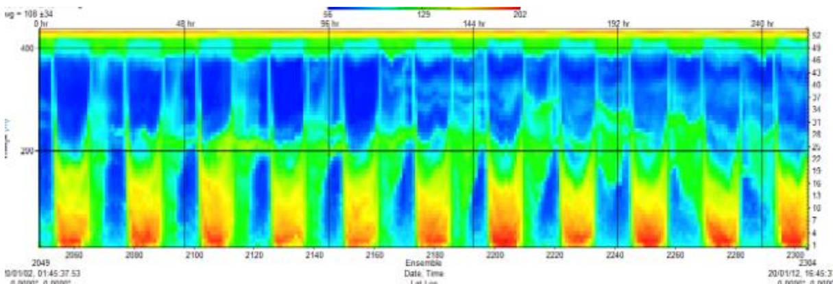
Figure 6-15. Upward-looking ADCP backscatter intensity plots (75 kHz) at 500 m depth from January 2 to January 12, 2020.
