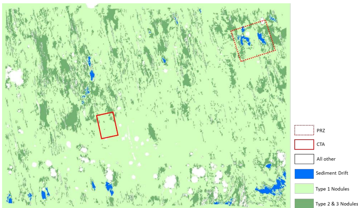
Figure 5-45. Location of CTA and PRZ in relation to nodule type on NORI-D
