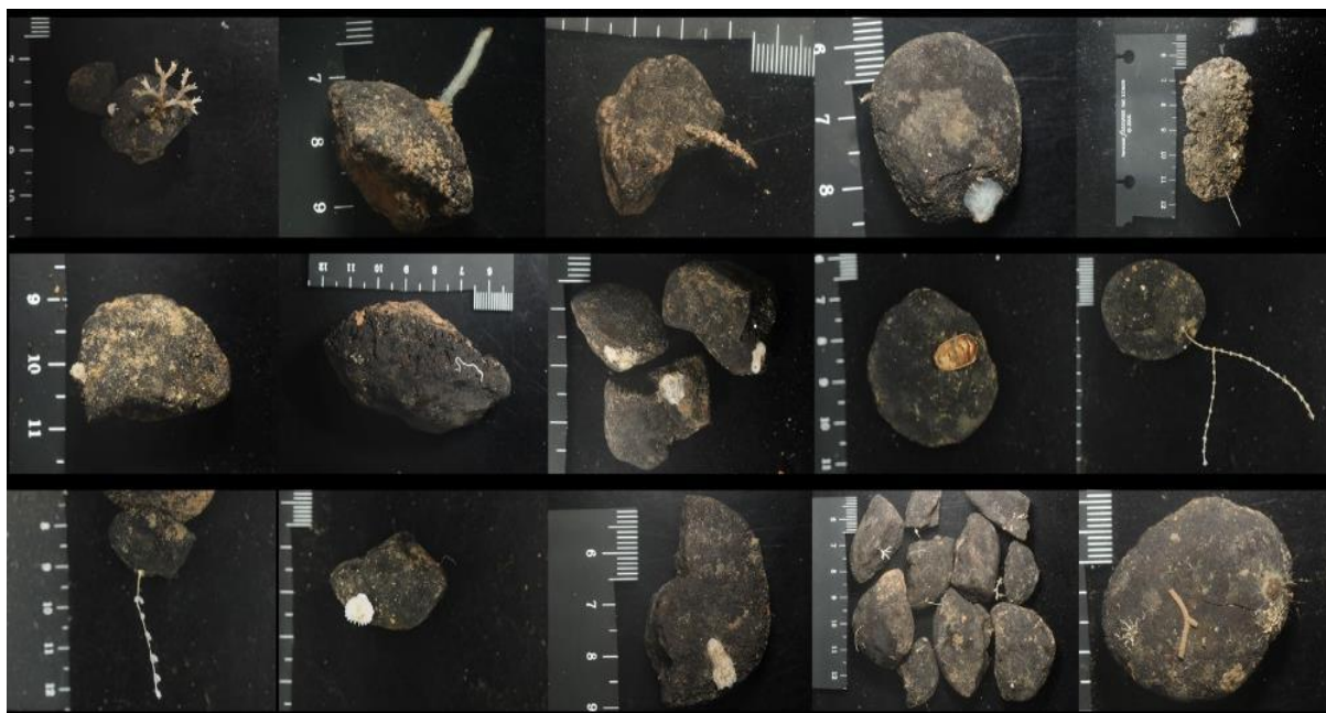
Figure 6-5. Images of the nodule fauna collected during Campaign 5A.
