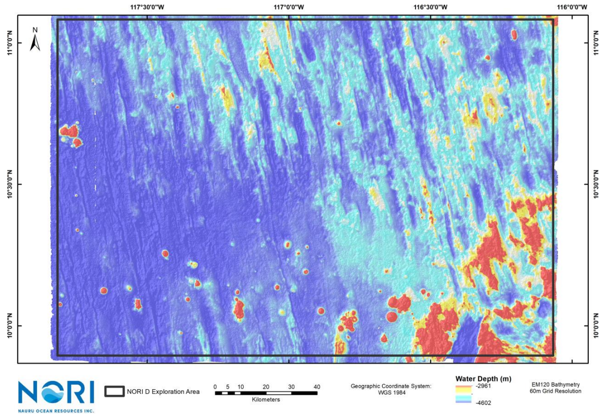
Figure 5-31. Bathymetry of NORI-D
