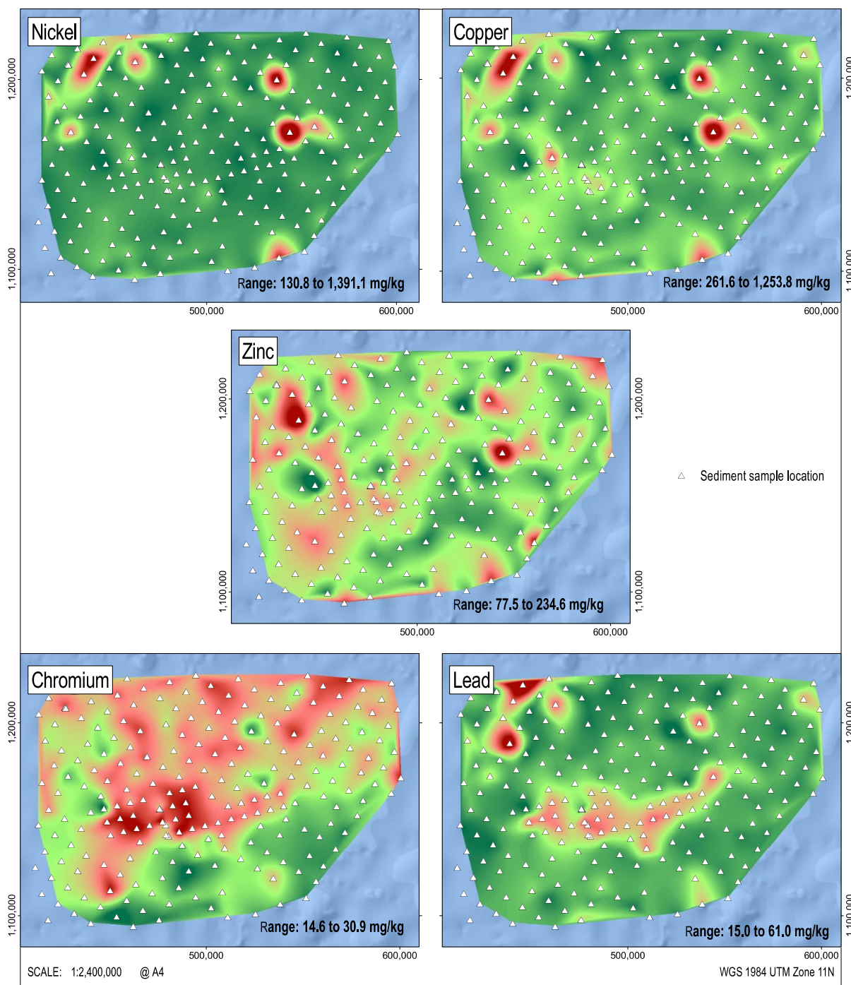
Figure 5-26. Relative variability of selected metal concentrations across NORI-D
