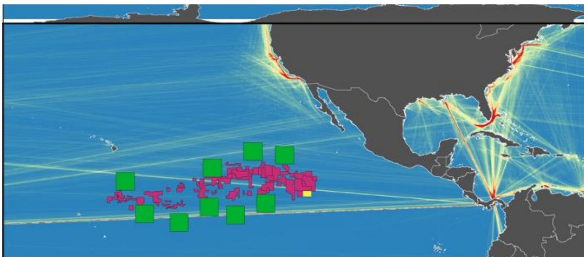
Figure 5-2. Shipping routes around the CCZ and NORI-D
