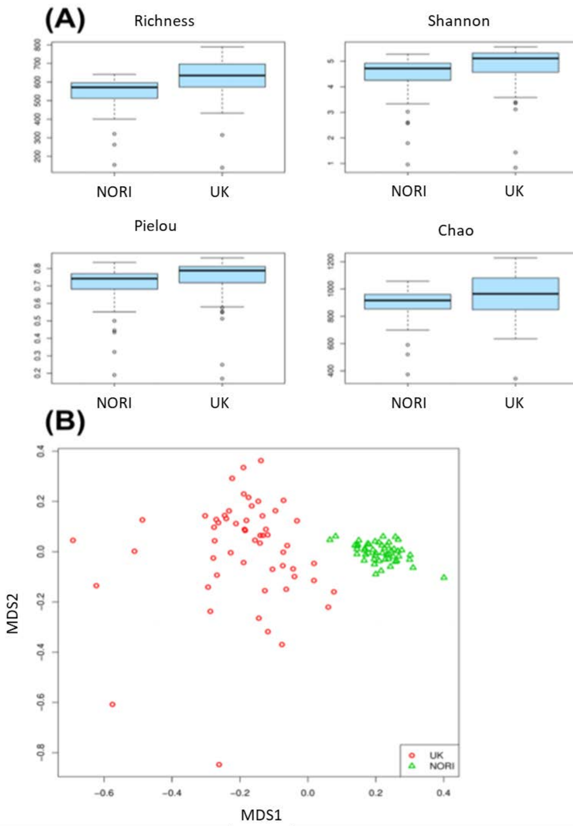
Figure 6-13. (A) alpha-diversity indices (B)NMDS calculated using V9 marker for UK area samples (red) and for NORI_D samples (green).
