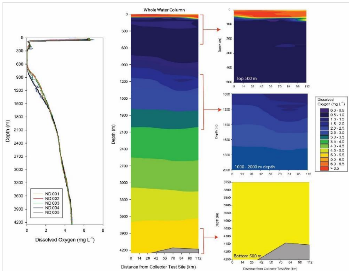
Figure 5-13. Dissolved oxygen profiles in the NORI-D, October 2019
