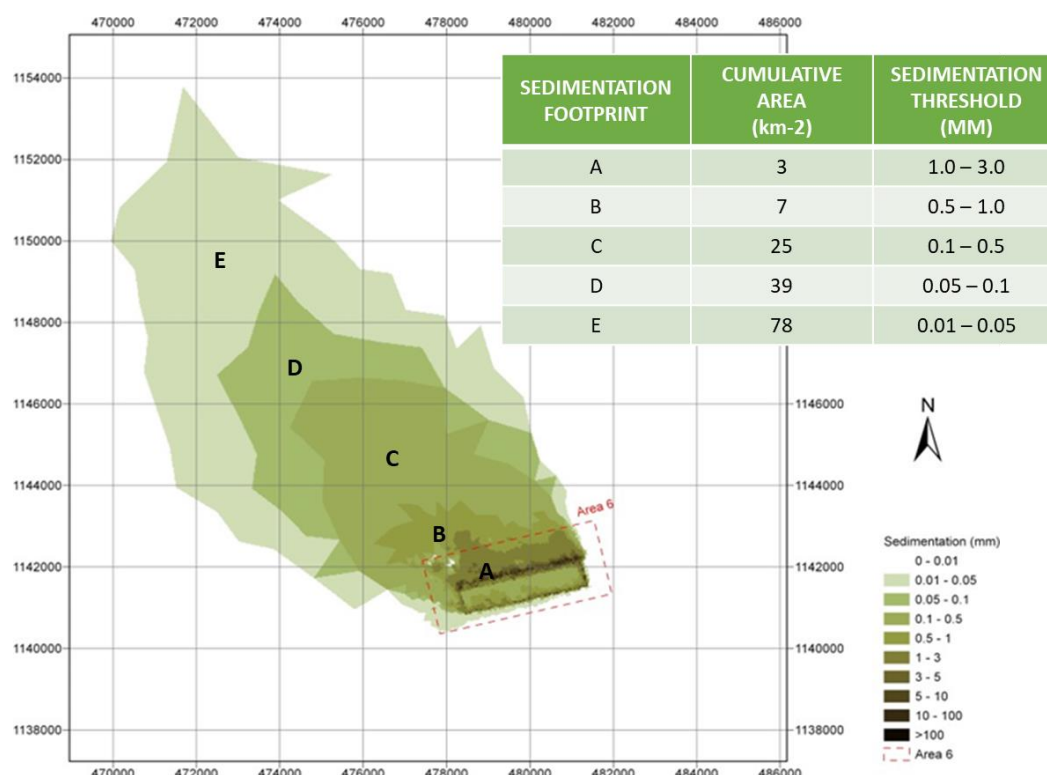
Figure 7-24. Benthic sedimentation footprints at various deposition depths
