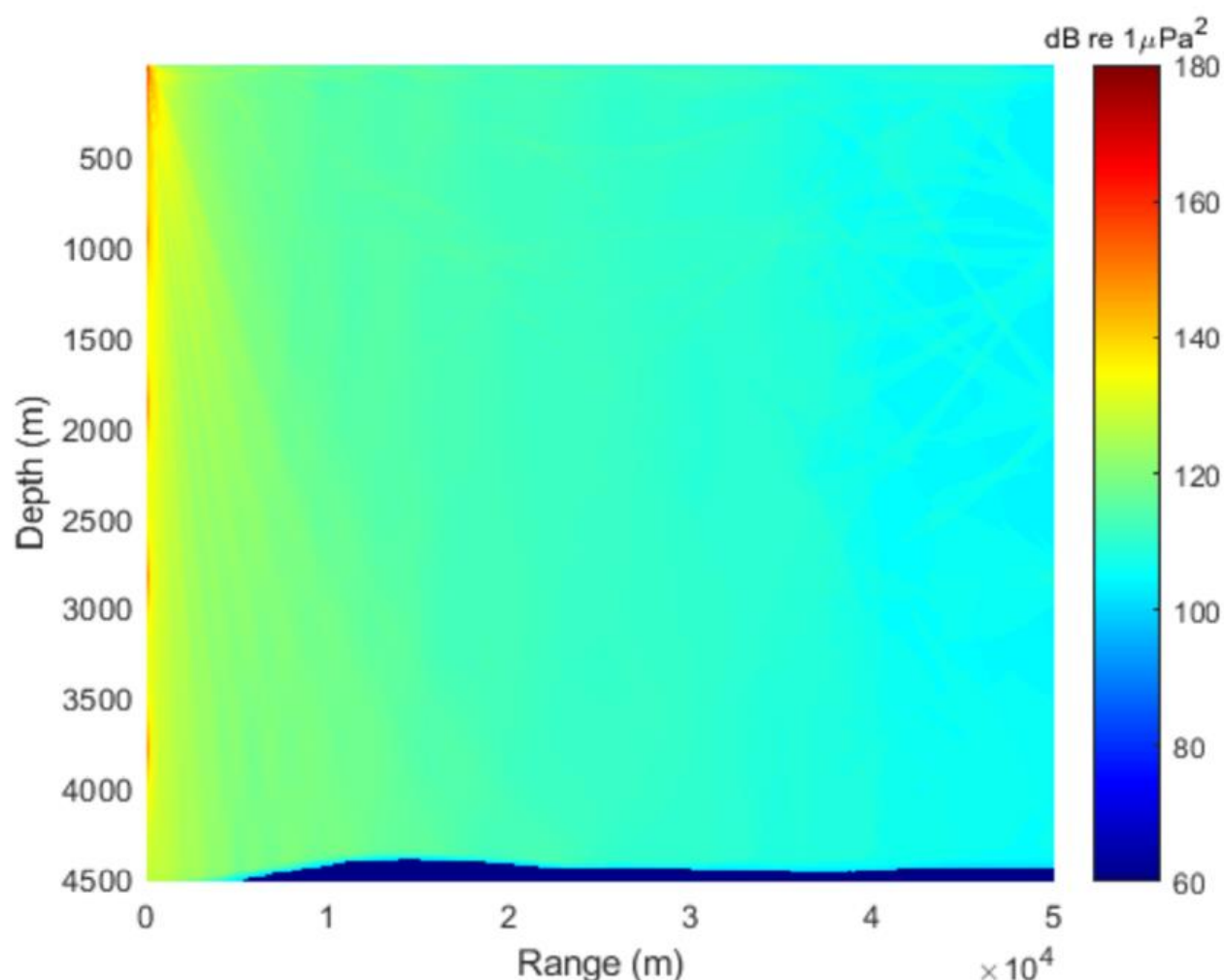
Figure 8-3. Sound pressure map for the Blue Nodule Project (van der Schaar et al. 2020)
