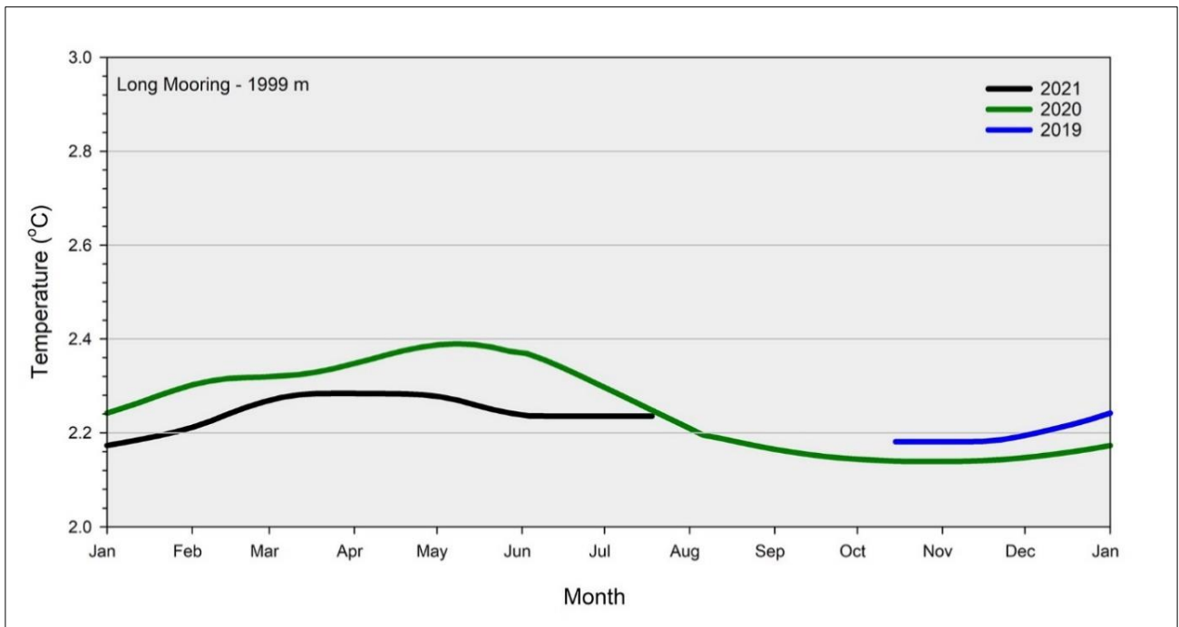
Figure 5-13. Running average of temperatures values (°C) by month at 2,000 m at the Long Mooring Site in the NORI-D block from October 2019 through July 2021.
