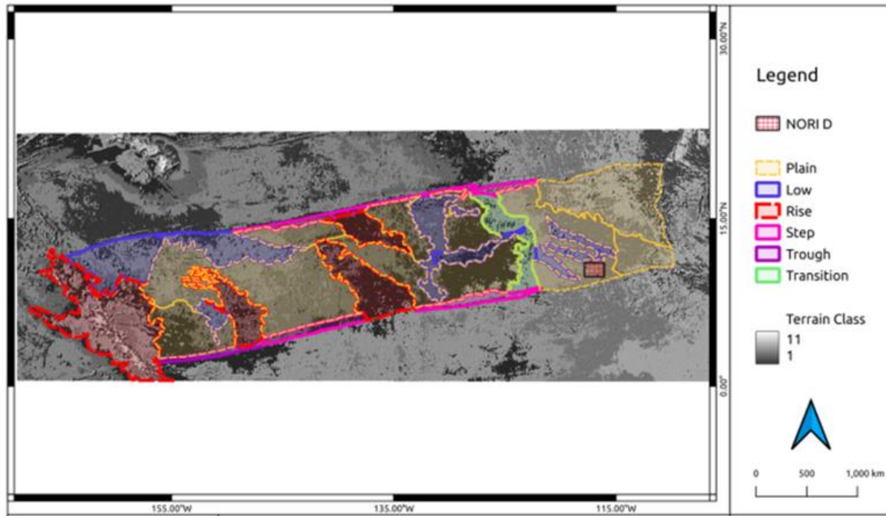
Figure 5-70. CCZ Level 1 classes of tectonic setting, geomorphology and algorithmic terrain classification.
