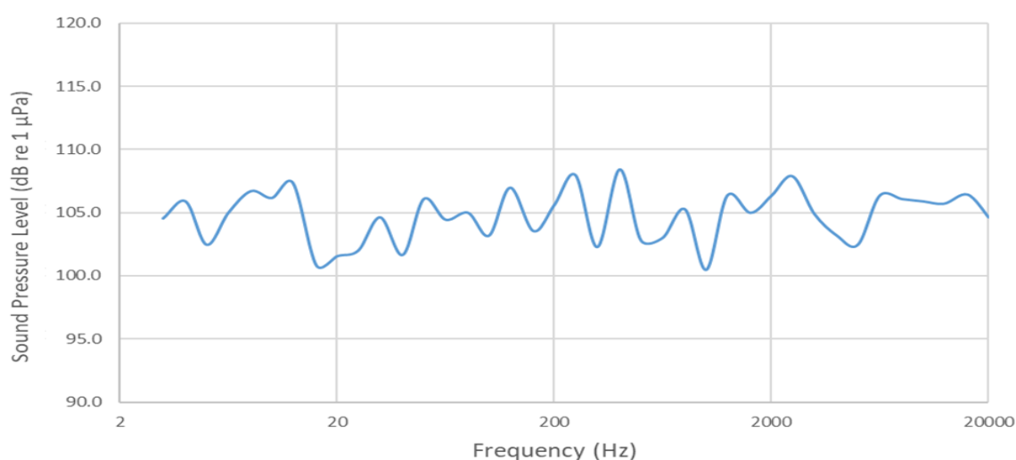
Figure 5-7. Power spectral density plot of the monthly averaged one-third octave spectrum from the shallow static acoustic recorder (SAR).
