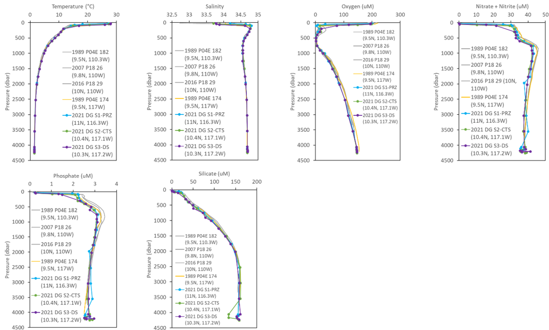
Figure 5-50. Full profiles of hydrographic data and nutrients in colour, atop historical data from the WOCE, CLIVAR, and GO-SHIP programs (cchdo.ucsd.edu). Historical data is shown in gray, except for the station nearest the NORI-D region, which is shown in yellow (but may have been sampled decades ago). All latitude/longitude data and the years of sampling are shown in the legends.
