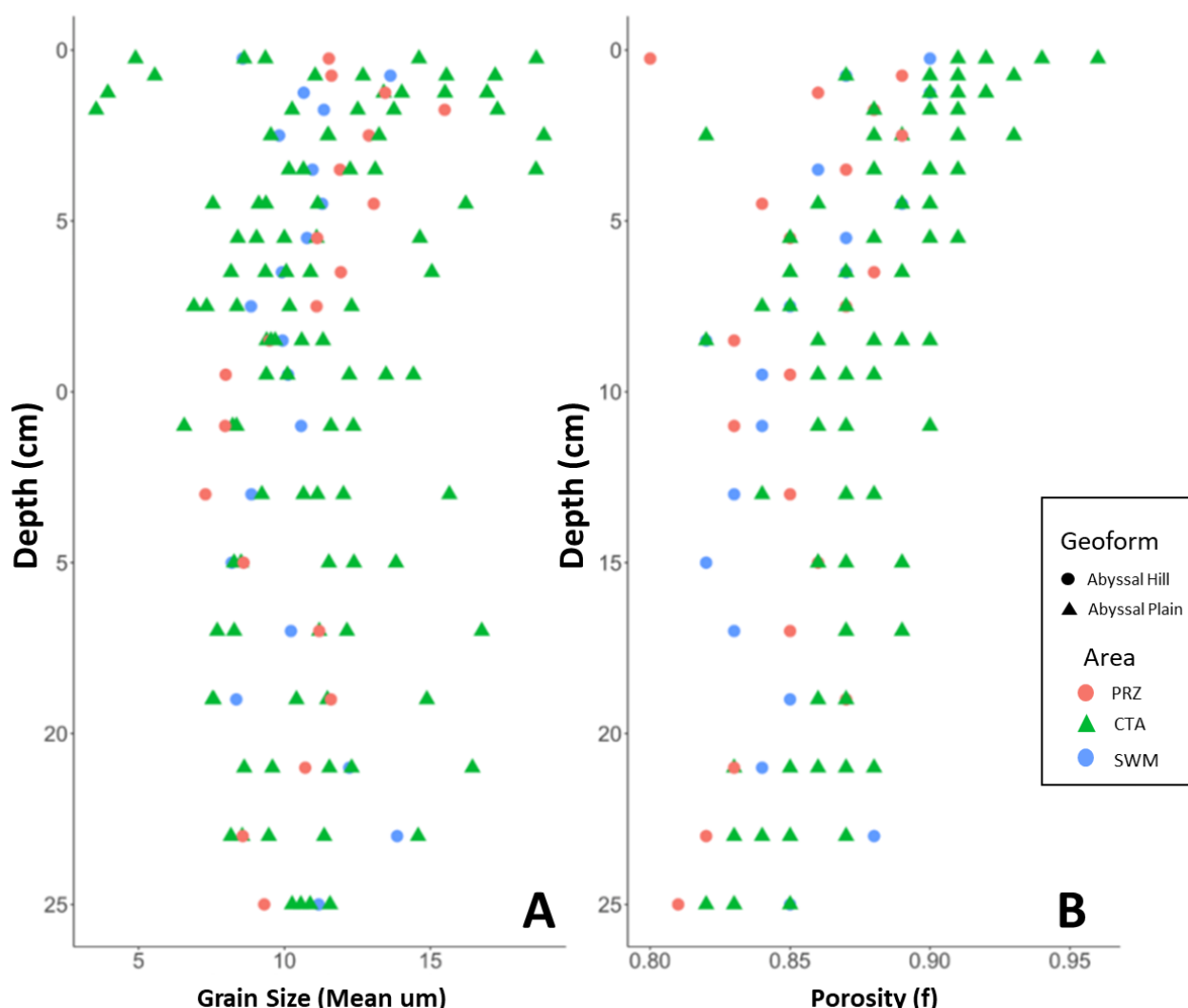
Figure 5-58. Mean grain size (A) and porosity (B) of sediment samples. Colours indicate sample region, shapes indicate geoform
