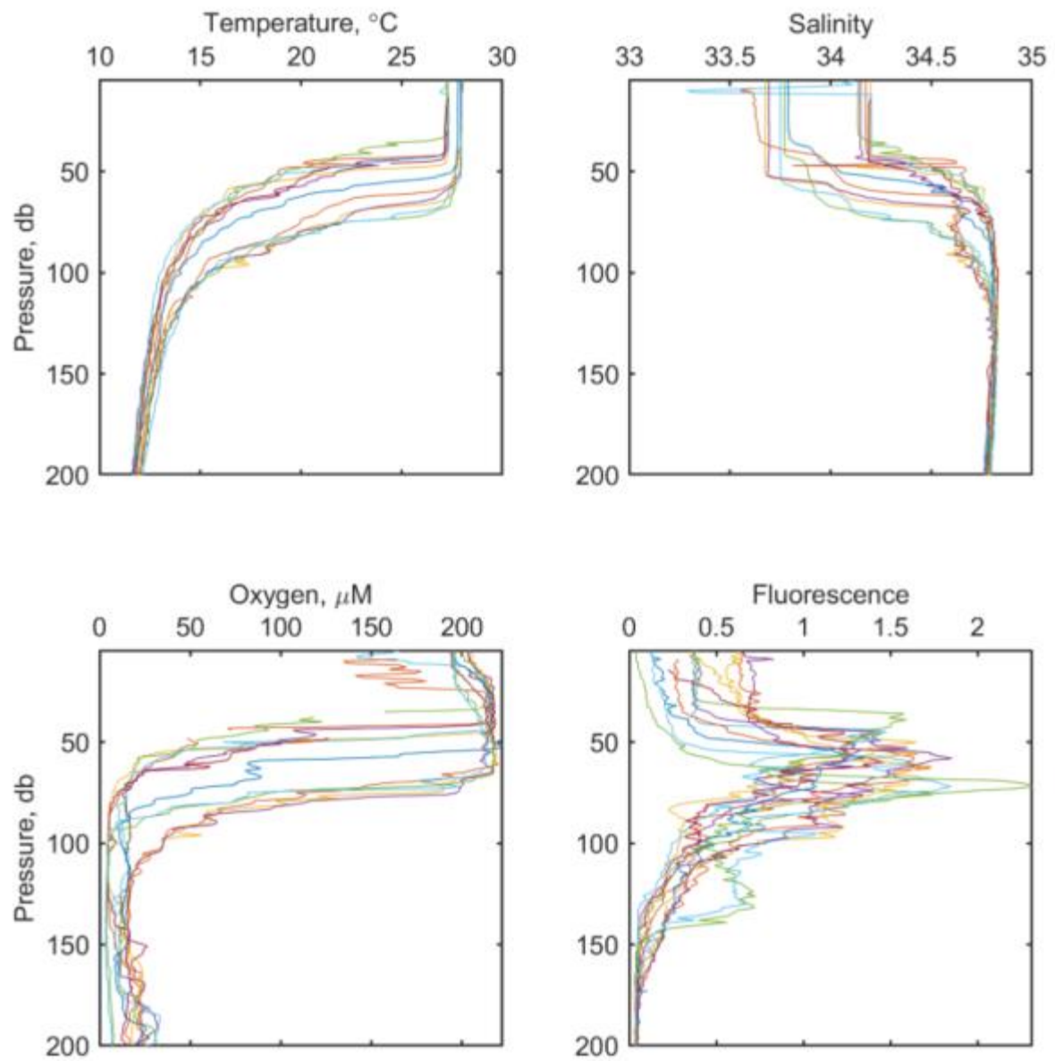
Figure 5-38. Vertical profiles of temperature, salinity, dissolved oxygen, and fluorescence in the upper 200 m of the water column at the PRZ site during Campaign 5B.
