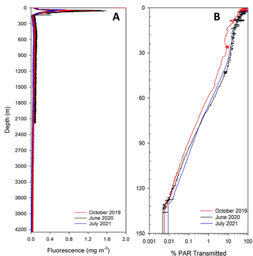
Figure 5-34. Average fluorescence and % photosynthetically active radiation (PAR) profiles among Campaign 4A – Oct'19, Campaign 4D – Jun'20, and Campaign 4E – Jul'21
