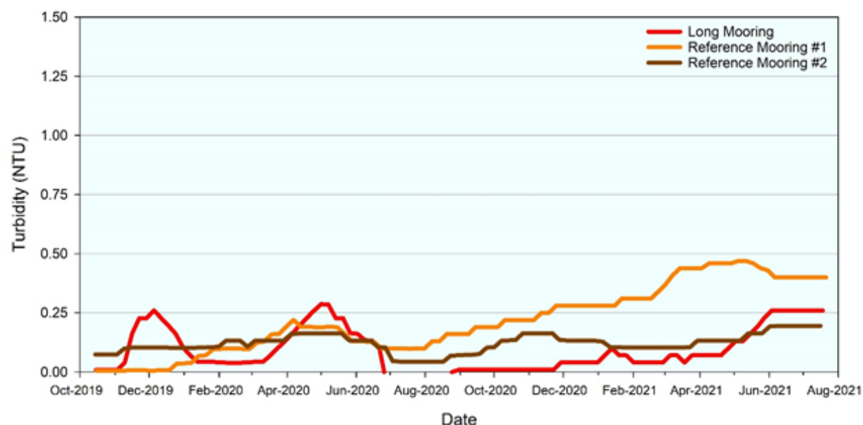
Figure 5-20. Running median of near-seafloor (i.e., <3.5 m above seafloor) turbidity values (NTU) at the Long (red) and Reference (orange and brown) mooring stations from October 2019 through July 2021.
