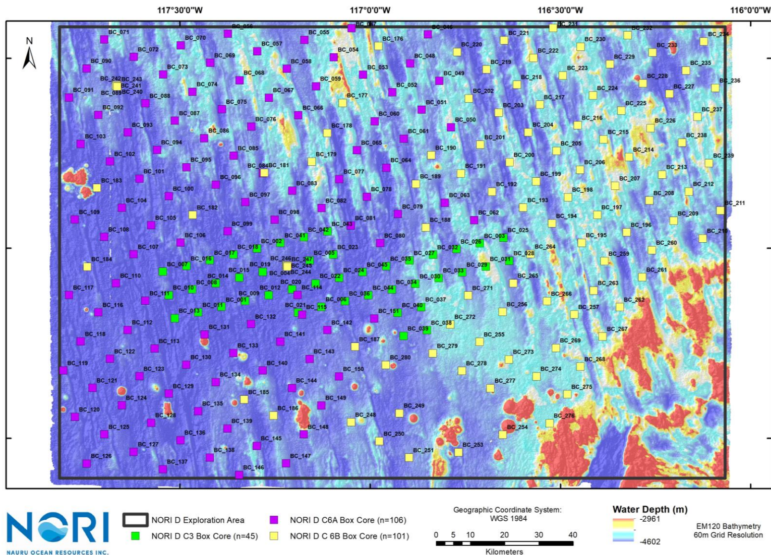
Figure 5-52. NORI-D seafloor sediment sampling locations
