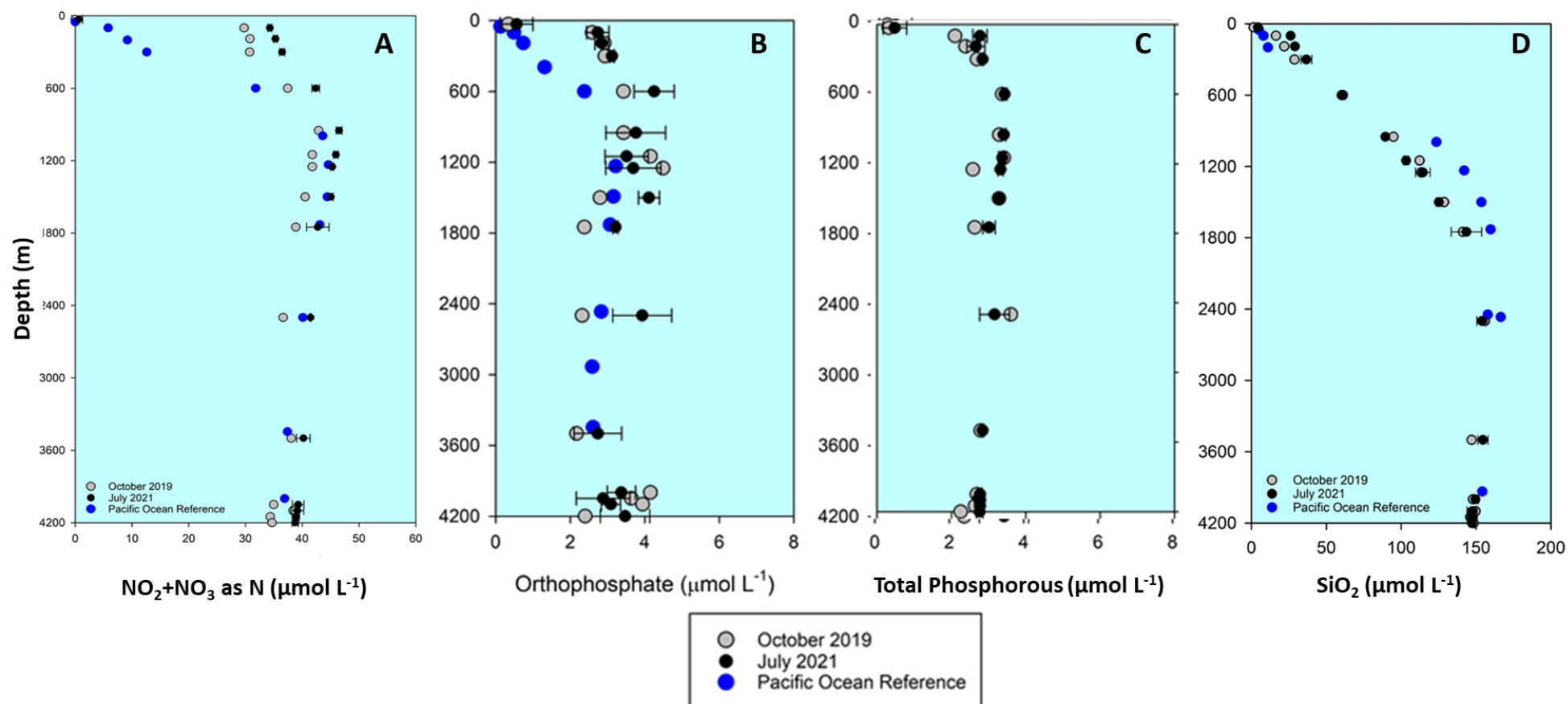
Figure 5-45. (A) - Average nitrogen ( \text{NO}_2 + \text{NO}_3^- ), (B) - orthophosphate ( \text{PO}_4 ), (C) - total phosphorous, and (D) - silicon dioxide ( \text{SiO}_2 ) concentrations within the NORI-D block during Campaigns 4A conducted in October 2019 (grey) and 4E conducted in July 2021 (black). Standard deviation bars are provided only for Campaign 4E. Blue symbols indicate general Pacific Ocean reference concentrations for orthophosphate from MBARI (2021).
