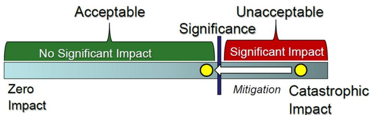
Figure 4-2. Significance spectrum (Ehrlich et al. , 2015)
