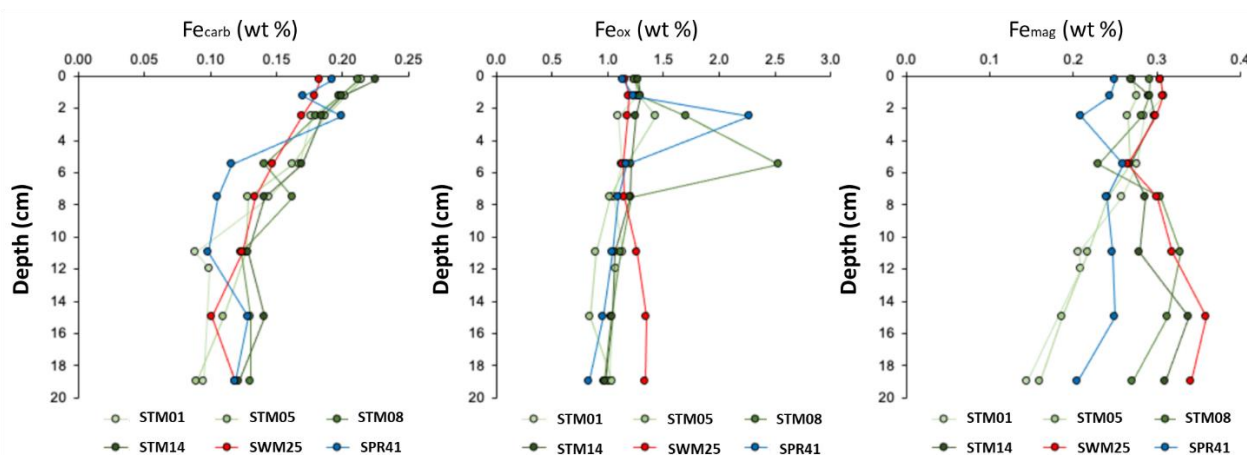
Figure 5-62. Fe mineral extractions from selected sites
