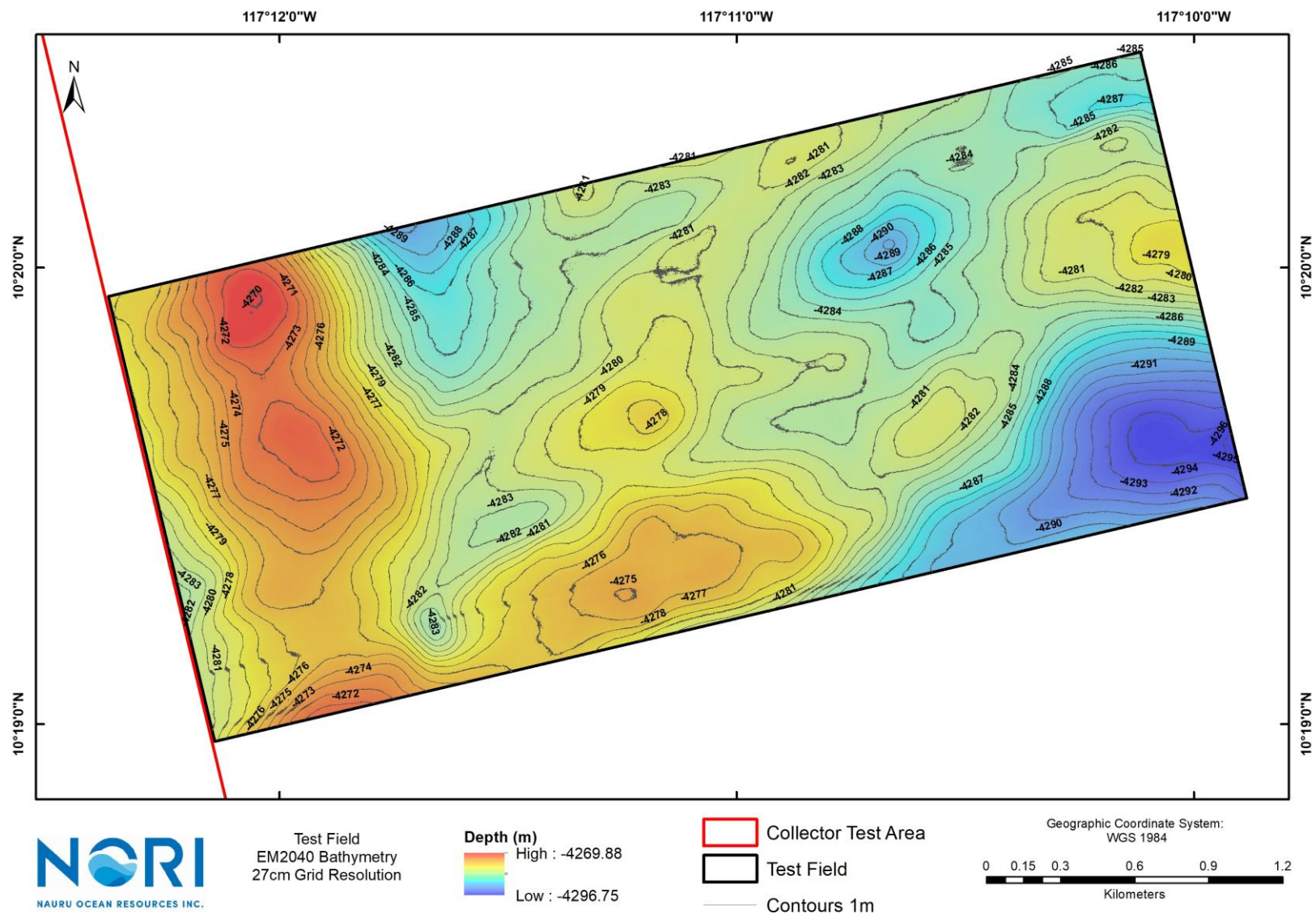
Figure 3-2. Test Field bathymetry (27cm grid)
