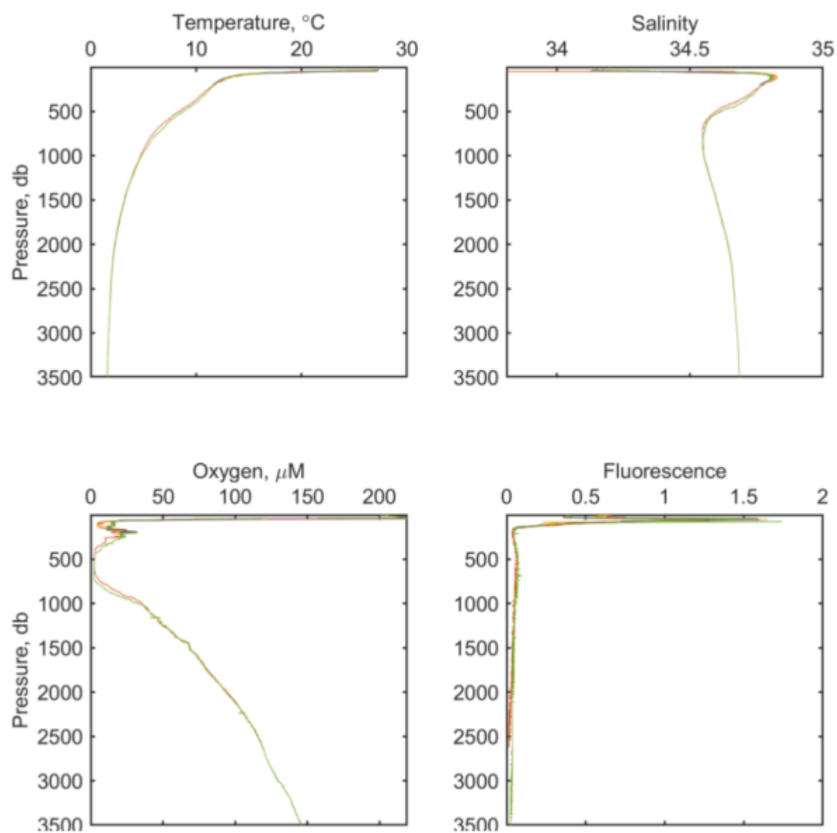
Figure 5-37. Vertical profiles of temperature, salinity, dissolved oxygen, and fluorescence measured with the regular CTD at the PRZ site during Campaign 5B.
