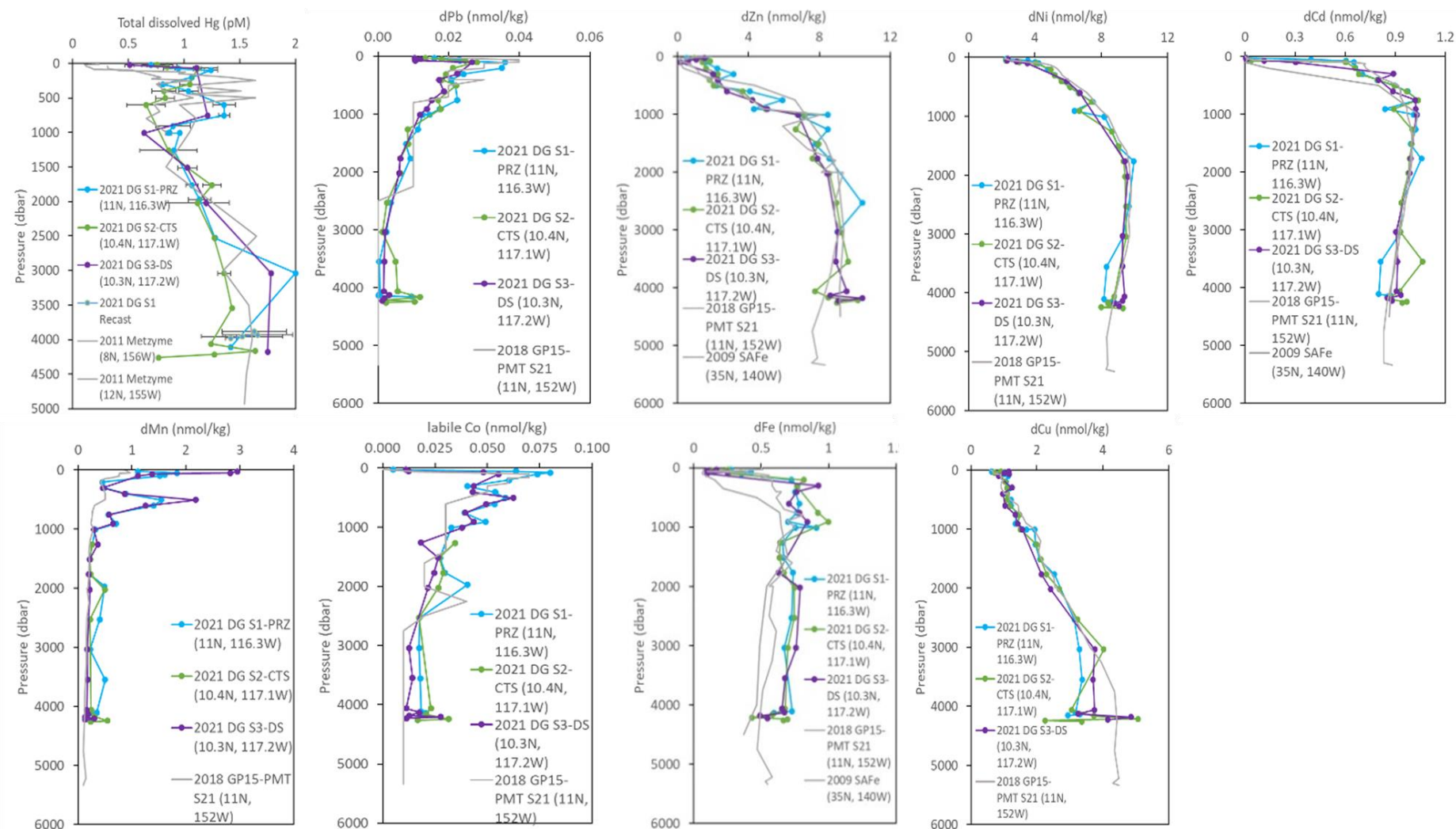
Figure 5-51. Full profiles dissolved metals and total dissolved Hg from Campaign 5B, atop historical data from other sites in the tropical/subtropical Pacific from the literature. Historical data is shown in gray. All latitude/longitude data and the years of sampling are shown in the legends. The literature total dissolved Hg data come from Munson et al. (2015), and some dissolved Fe, Zn, and Cd data come from Conway and John (2015). The rest of the dissolved metals data is unpublished from the GEOTRACES GP15-PMT cruise (Fitzsimmons, unpublished) and should be considered preliminary.
