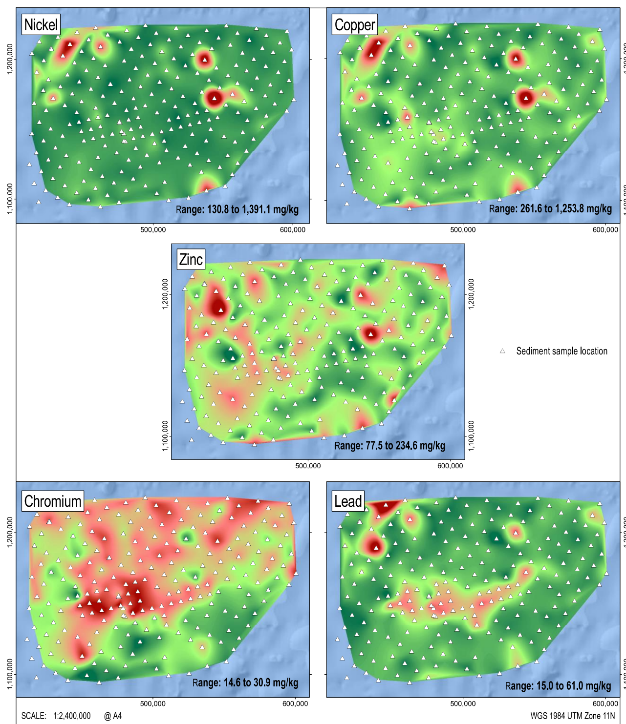
Figure 5-53. Relative variability of selected metal concentrations across NORI-D
