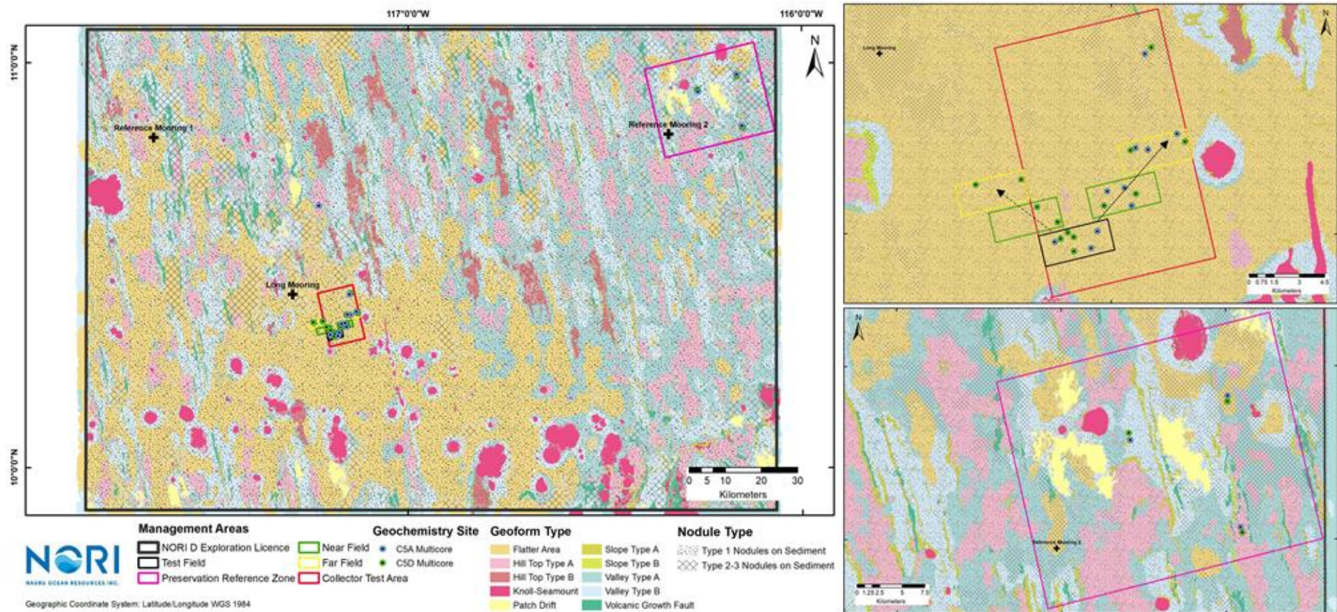
Figure 5-54. Sediment geochemistry sample sites - Campaign 5A and 5D
