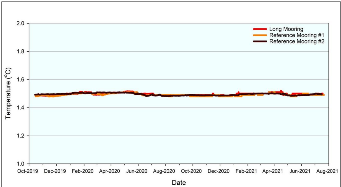
Figure 5-13. Running average of temperatures values (°C) by month at 2,000 m at the Long Mooring Site in the NORI-D block from October 2019 through July 2021.
