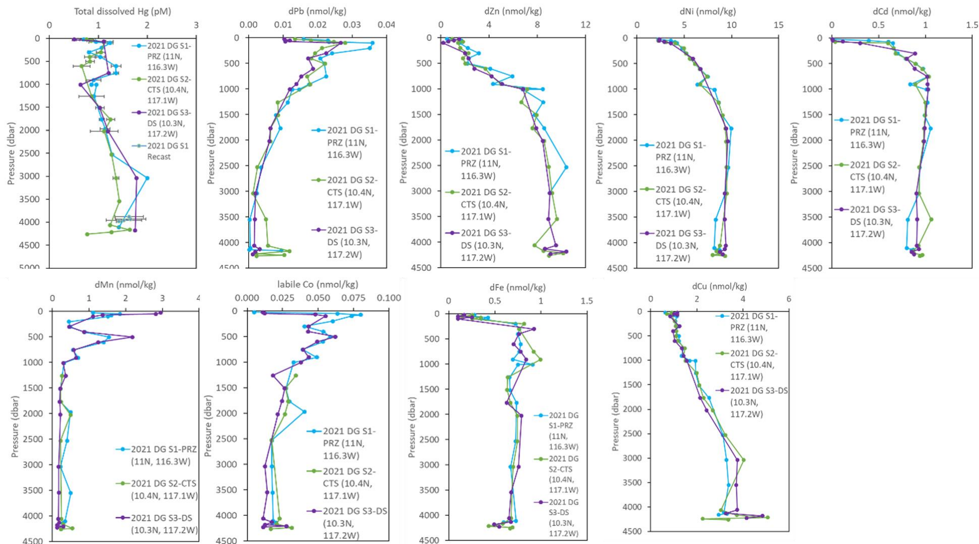
Figure 5-48. Dissolved concentrations of mercury, lead, zinc, nickel, cadmium, manganese, labile cobalt, iron and copper at PRZ, CTA and downstream CTA (pending QA/QC)
