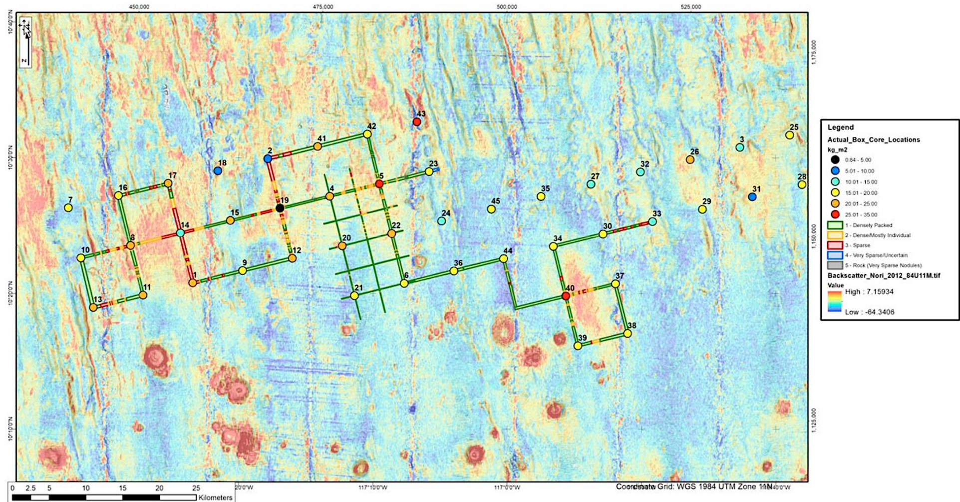
Figure 5-68. Nodule classification in NORI-D
