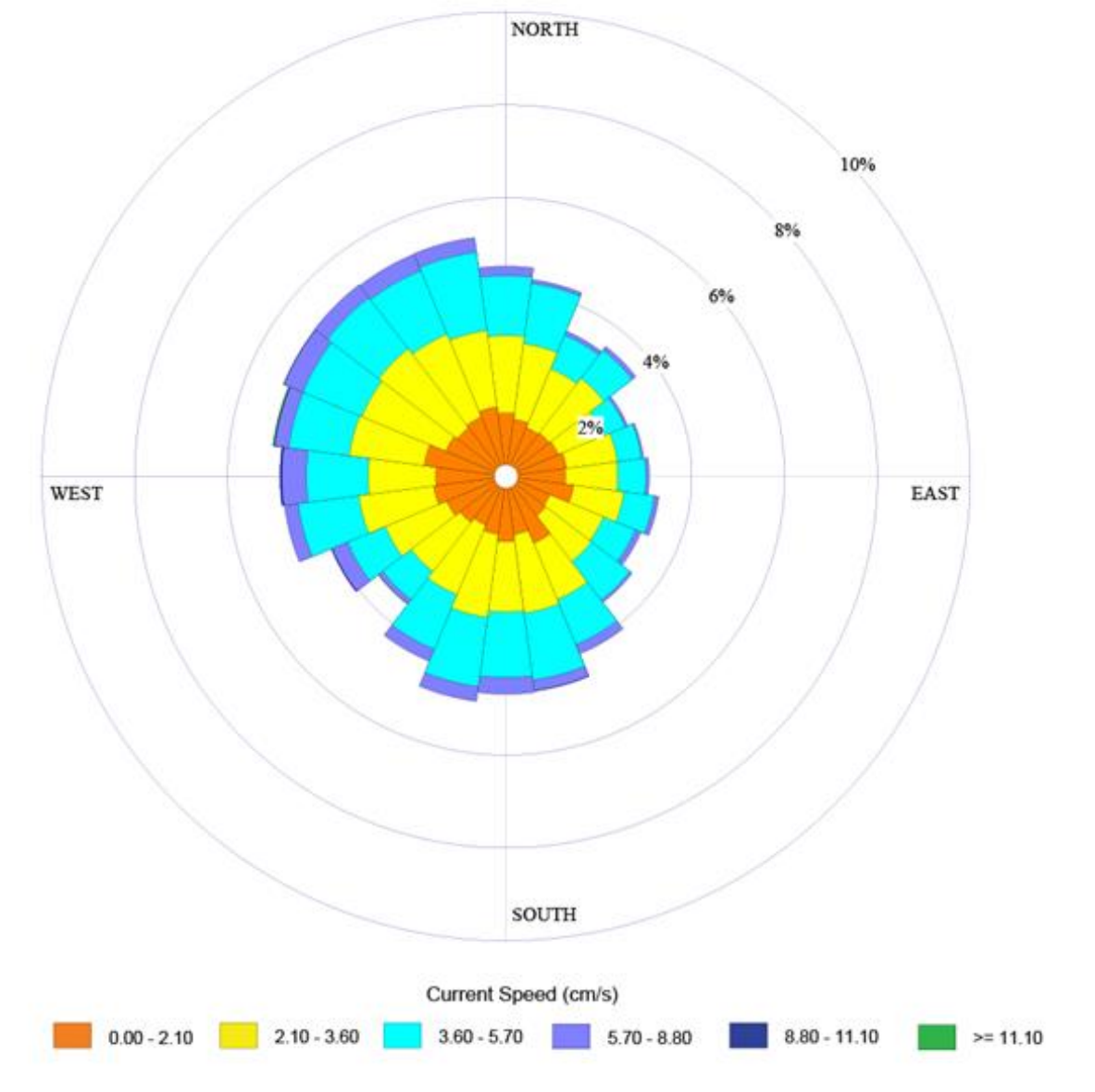
Figure 5-27. Near-continuous record of current speeds (cm s -1 ) and direction (flowing towards) recorded from bin #4 of the downward looking Acoustic Doppler Current Profiler (ADCP) (600 kHz) at 4,321 m water depth (i.e., 5 m above the seafloor) on the Long Mooring.
