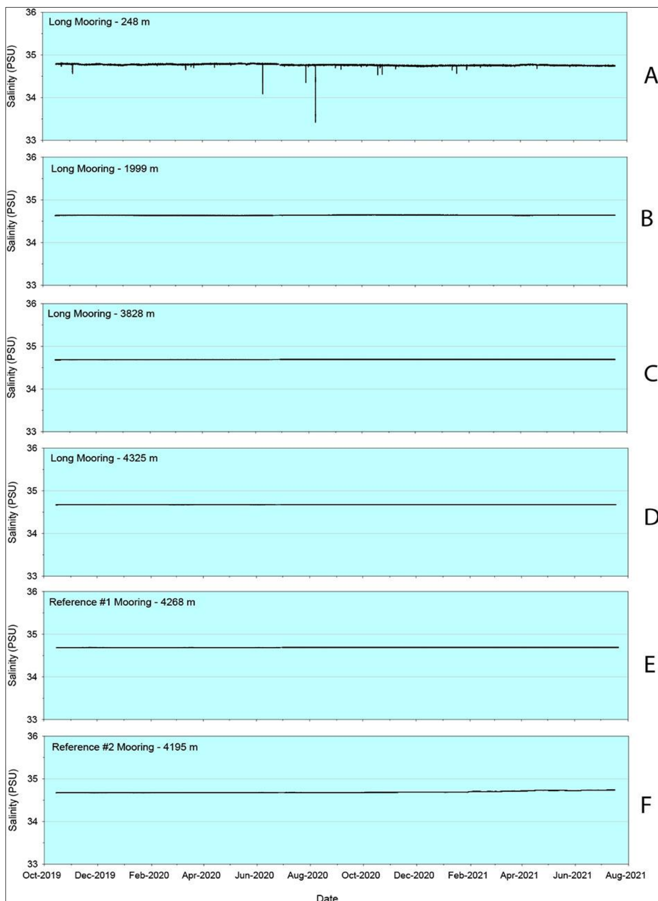
Figure 5-14. Near-continuous salinity values (PSU) at selected Long (A to D) and Reference (E to F) mooring conductivity-temperature-depth (CTD) instrumentation depths in the NORI-D block from October 2019 through July 2021.
