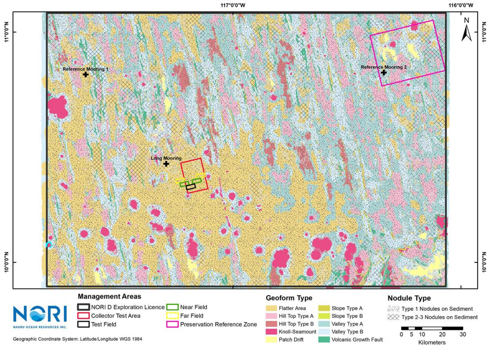
Figure 5-72. NORI-D Level 3 geoforms and Level 3 substrates
