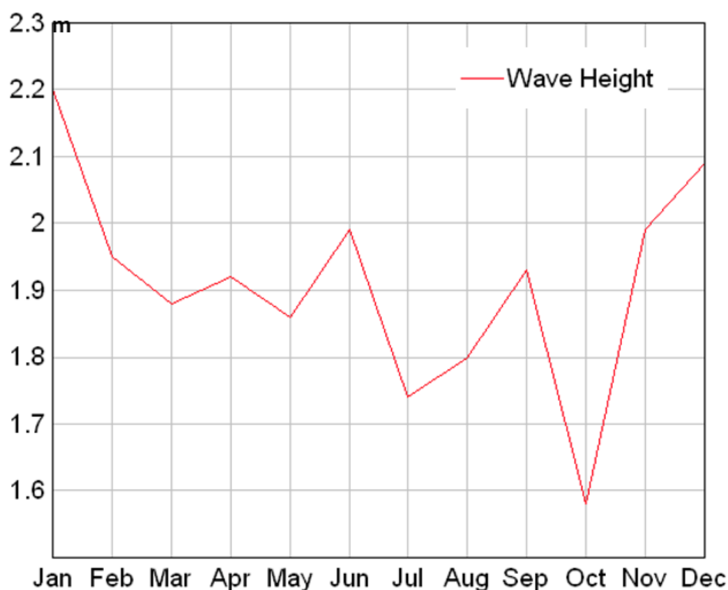
Figure 5-8. Average monthly wave heights in the CCZ
