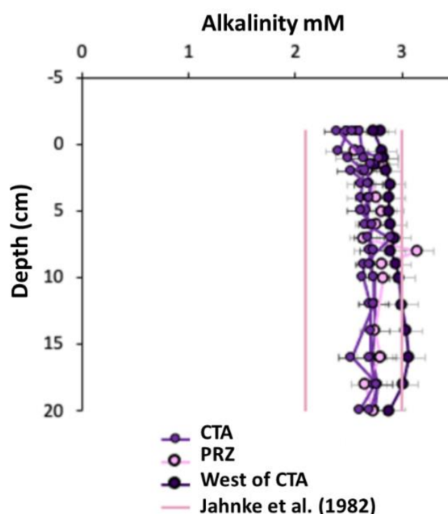
Figure 5-57. Porewater alkalinity results colour coded for sampling region.
