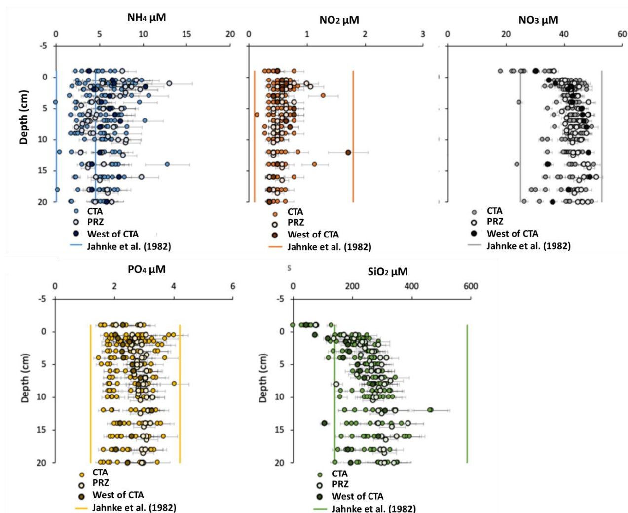
Figure 5-55. Porewater concentrations of nutrients colour coded for sample area.
