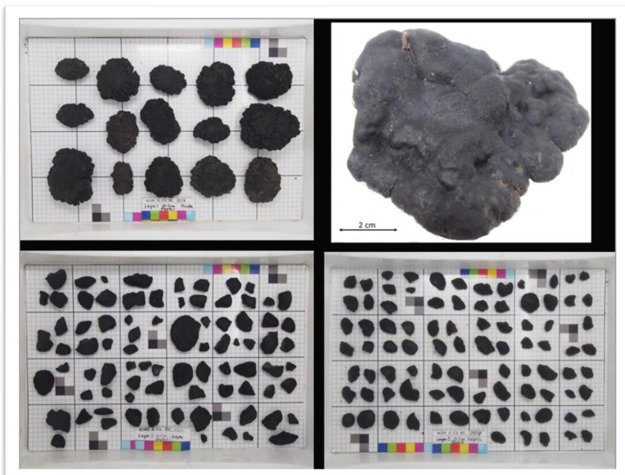
Figure 5-67. NORI-D nodule collection showing ranges of sizes
