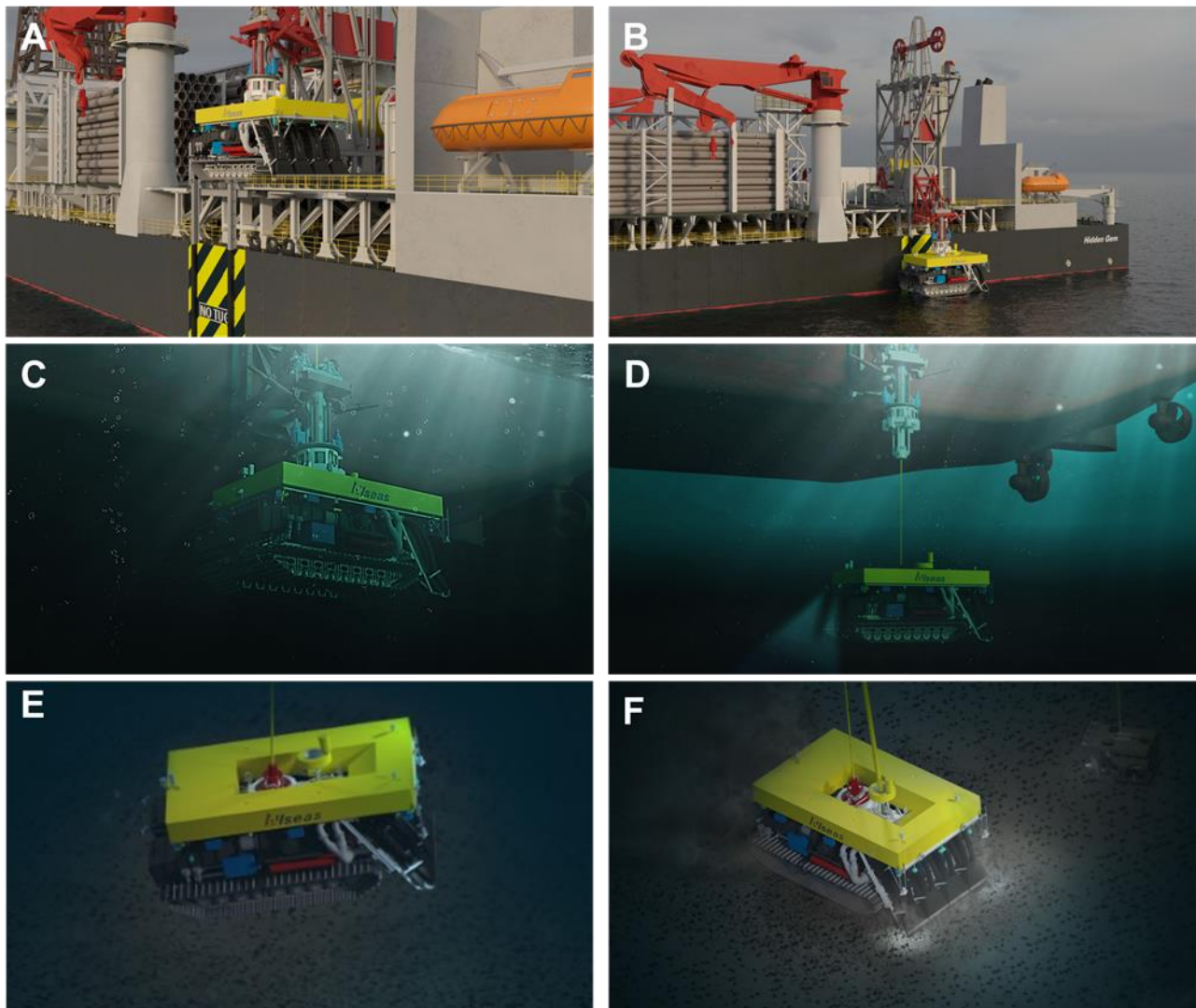
Figure 3-22. PCV deployment & recovery sequence
