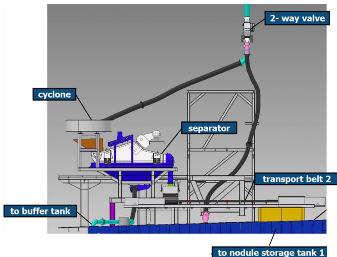
Figure 3-13. Side view of surface process flow equipment
