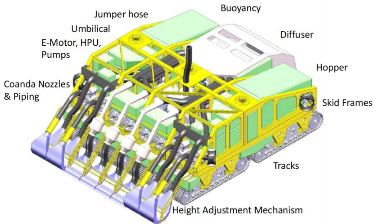
Figure 3-8 Main components of the Prototype Collector Vehicle
