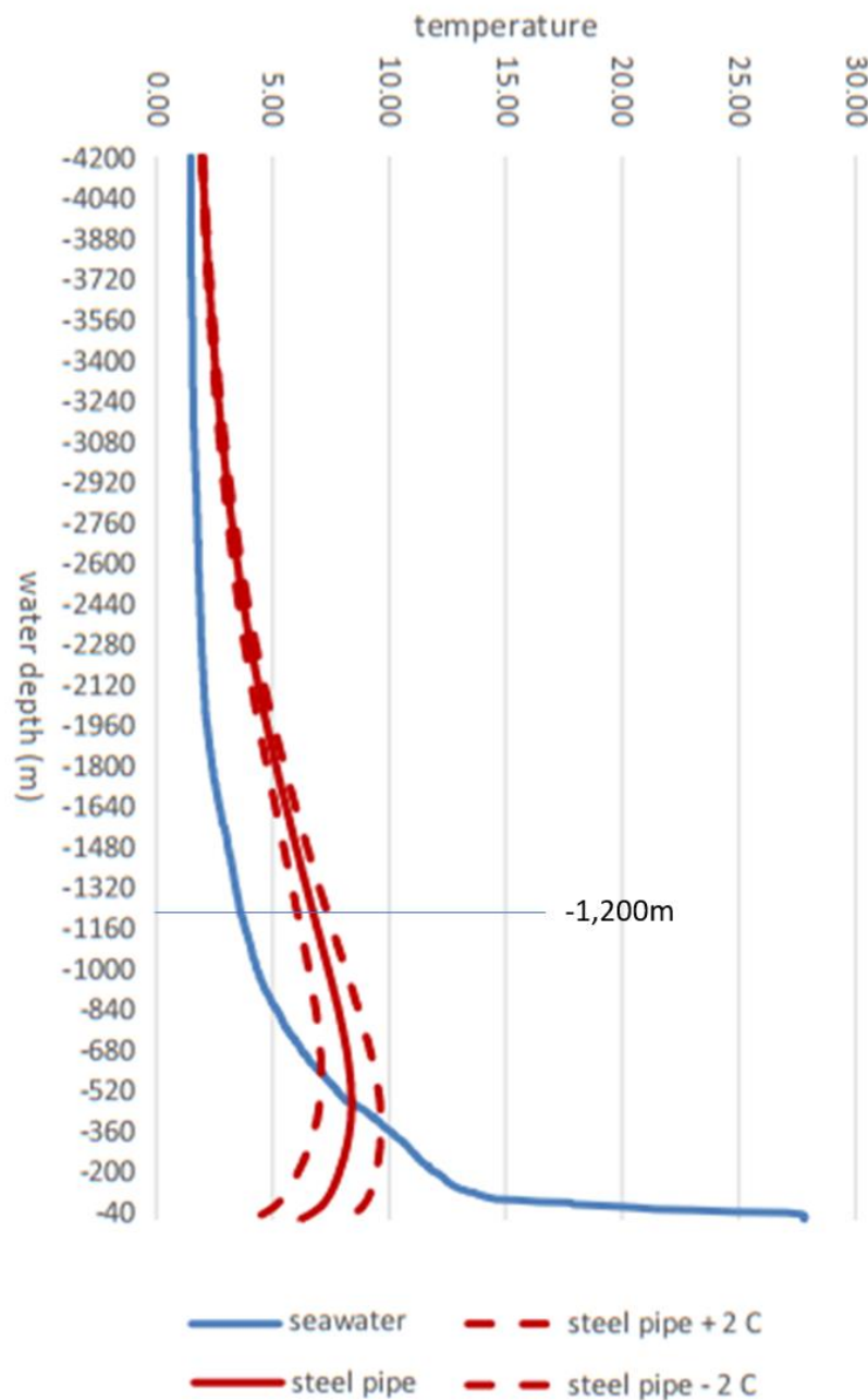
Figure 3-16. Modelled return water temperature and ambient seawater temperature (°C) at depth (m)
