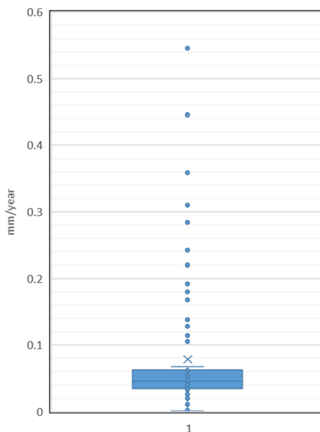
Figure 5-30. Near bed sediment trap data from NORI-D area, October 2019 to June 2021 converted to sedimentation rate based on a density of 180kg/m 3
