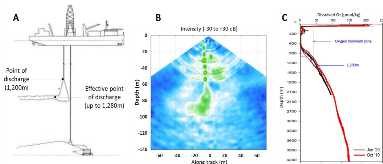
Figure 3-15. A - Effective point of discharge; B – PLUMEX modelling; C – Oxygen profile for NORI-D
