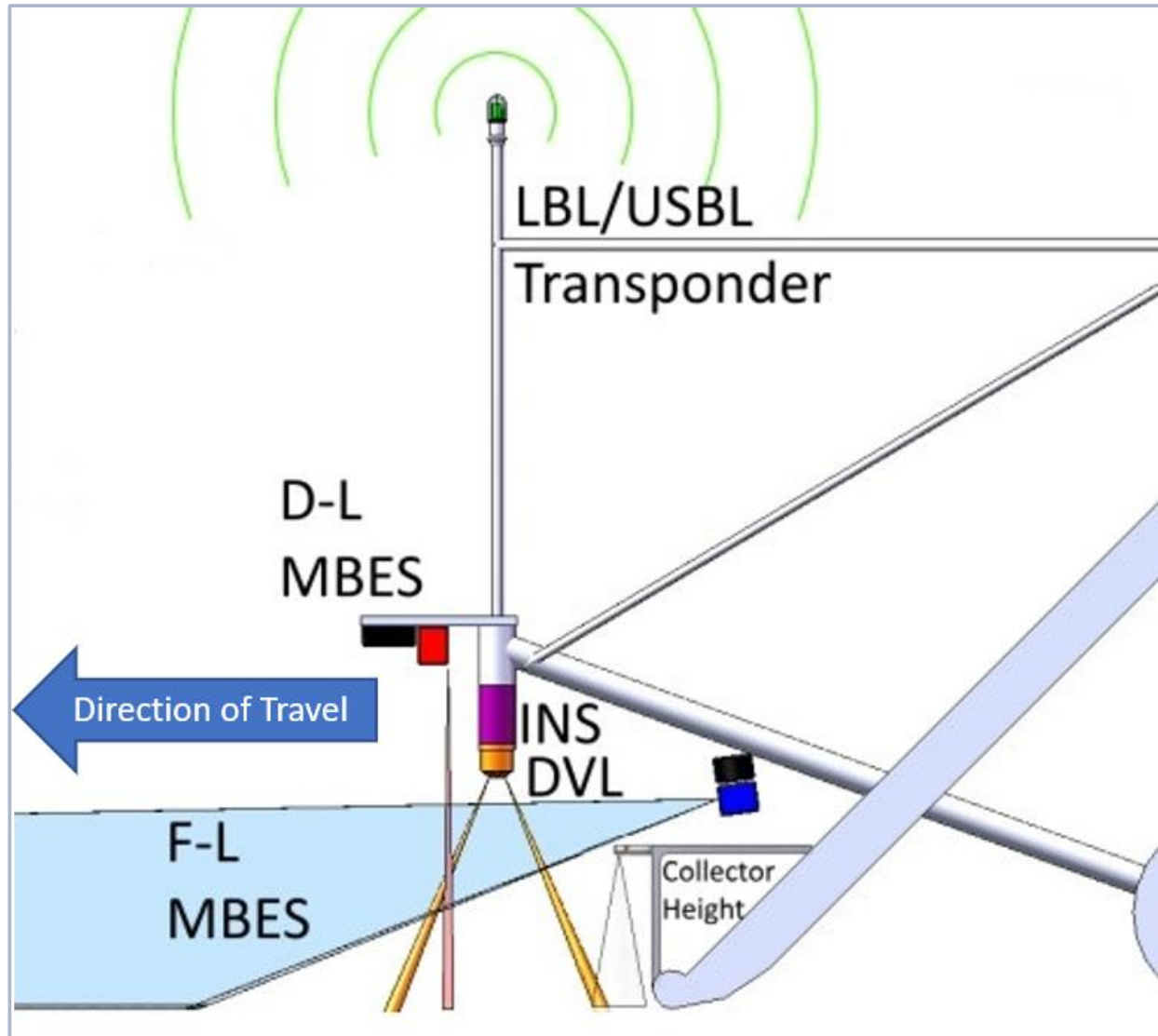
Figure 3-20. PCV navigation system
