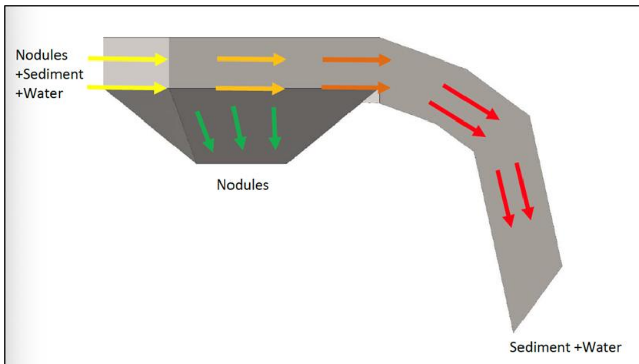
Figure 3-11. General layout of nodule processing system
