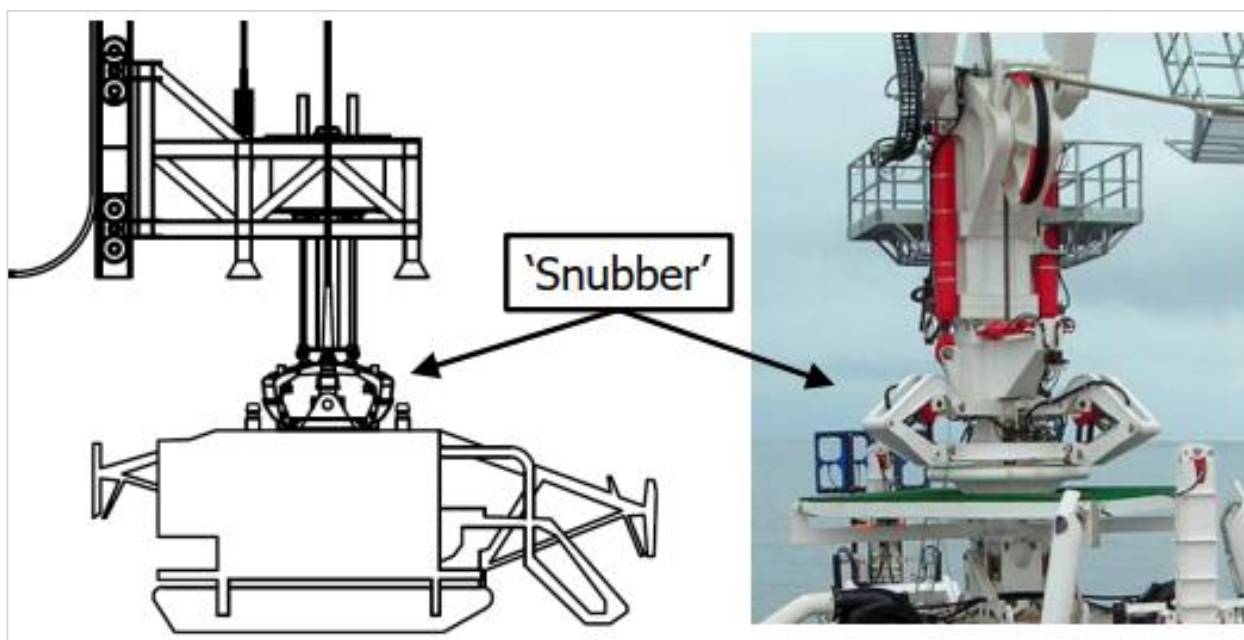
Figure 3-21. Snubber configuration
