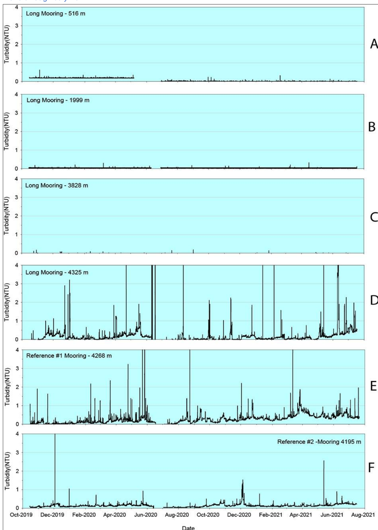
Figure 5-18. Near-continuous turbidity values (NTU) at selected Long (A to D) and Reference (E to F) mooring conductivity-temperature-depth (CTD) instrumentation depths in the NORI-D block from October 2019 through July 2021.
