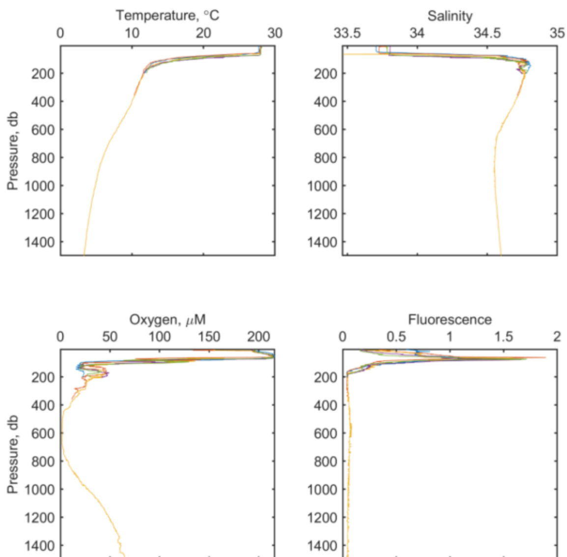
Figure 5-39. Vertical profiles of temperature, salinity, dissolved oxygen, and fluorescence measured with the regular CTD at the CTA site during campaign 5B.
