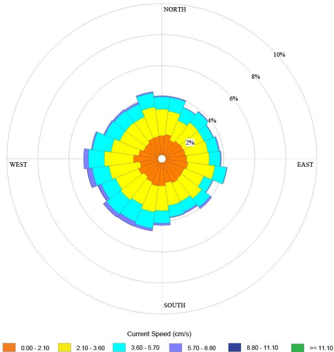
Figure 5-23. Near-continuous record of current speeds (cm s -1 ) and direction (flowing towards) recorded from bin #4 of upward-looking acoustic Doppler current profiler (ADCP) (300 kHz) at 2,000 m on the Long Mooring between 15 October 2019 and 2 June 2021.
