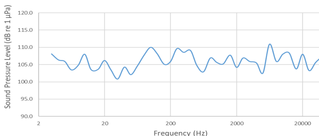
Figure 5-7. Power spectral density plot of the monthly averaged one-third octave spectrum from the shallow static acoustic recorder (SAR).
