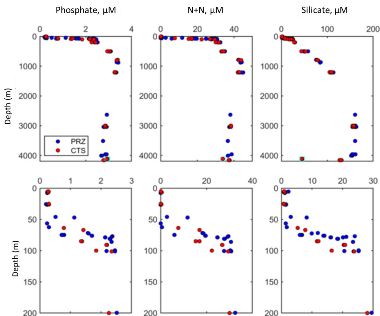
Figure 5-47. Vertical profiles of phosphate, nitrate plus nitrite (N+N) and silicate concentrations at across NORI-D collected on Campaign 4A and 5B
