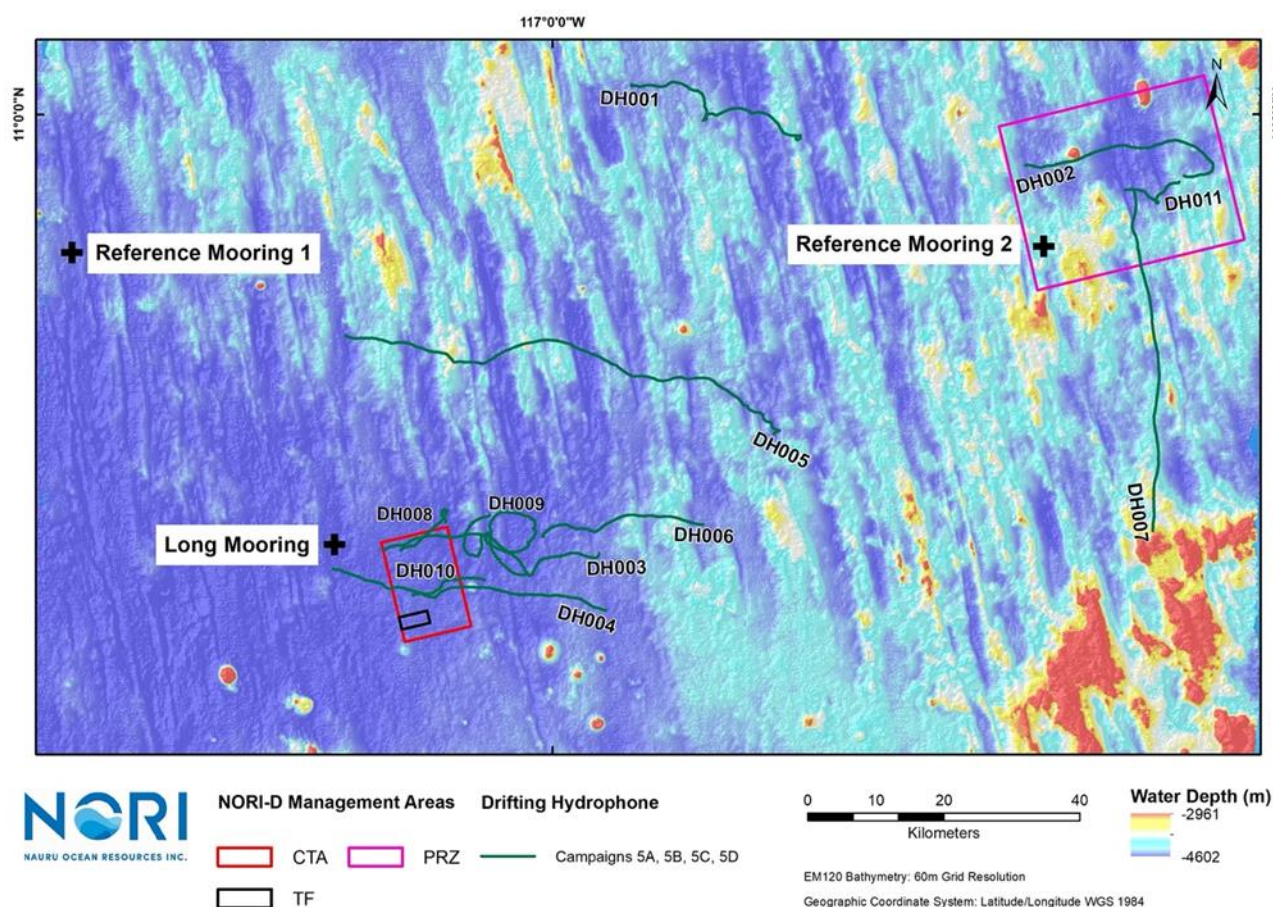
Figure 5-3. Long mooring location and tracks of the hydrophone drifting array from campaigns 5A, 5B and 5D 3
