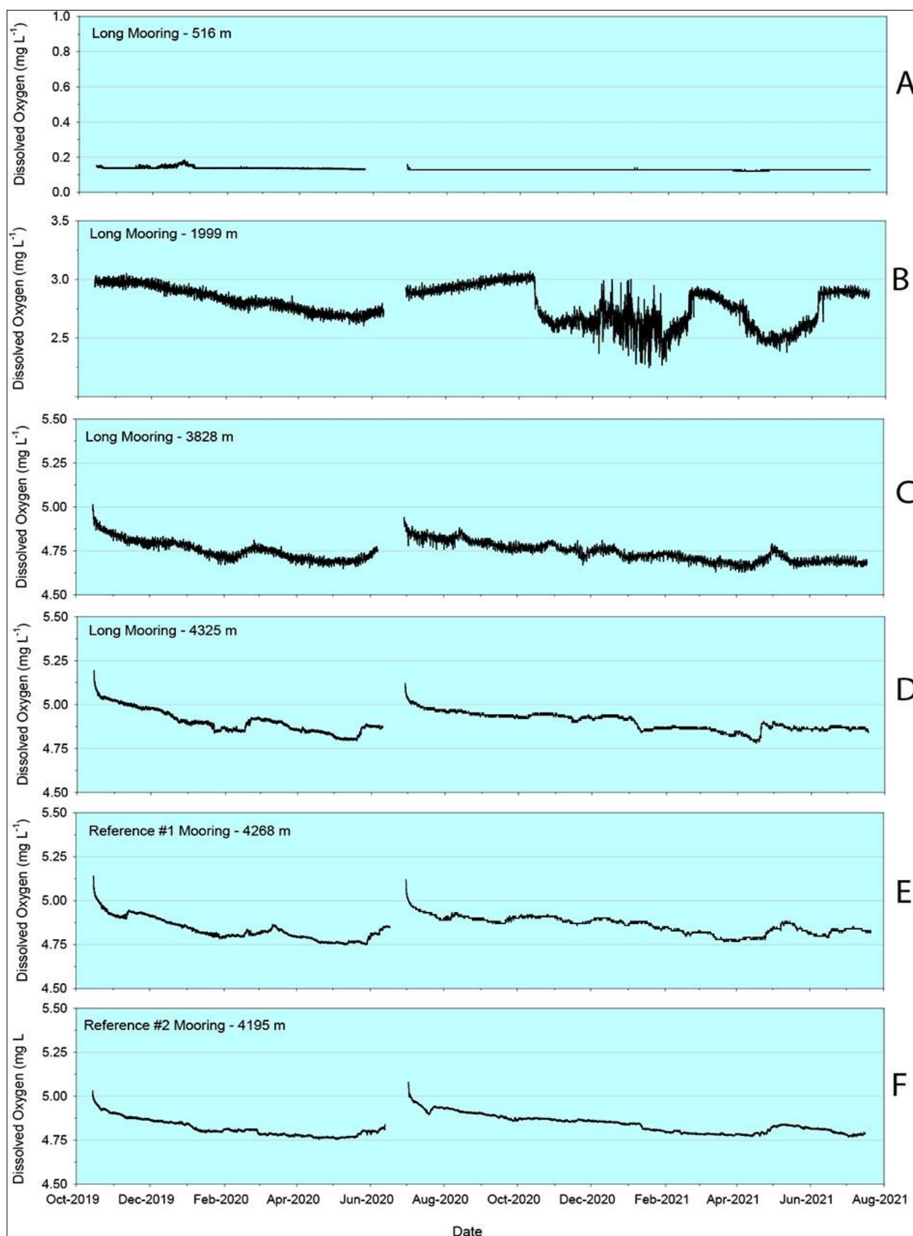
Figure 5-15. Near-continuous dissolved oxygen values (mg L -1 ) at selected Long (A to D) and Reference (E to F) mooring conductivity-temperature-depth (CTD) instrumentation depths in the NORI D block from October 2019 through July 2021. Note the difference in y-axis scales.
