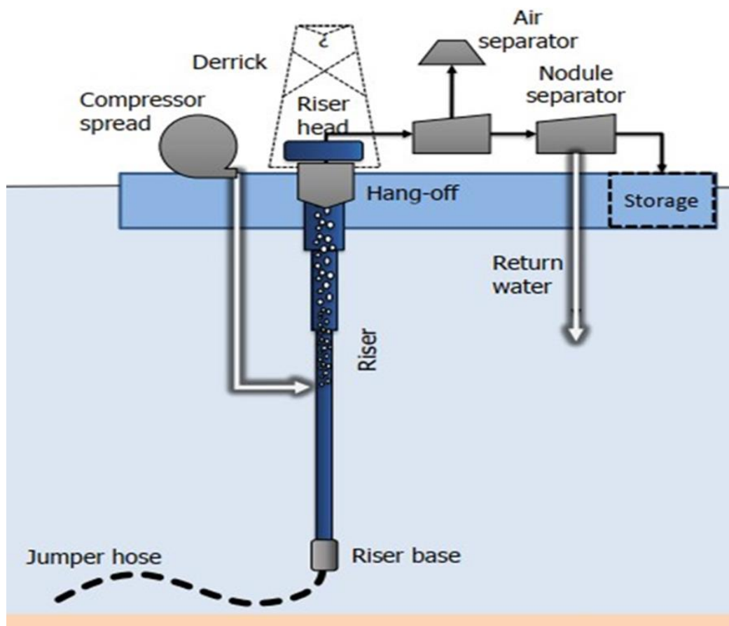
Figure 3-12. Air lift system
