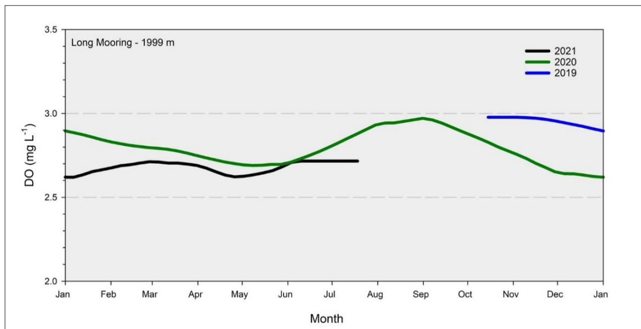
Figure 5-17. Running average of dissolved oxygen concentration values (mg L -1 ) by month at the proposed discharge water depth (~2,000 m) at the Long Mooring Site in the NORI-D block from October 2019 through July 2021.
