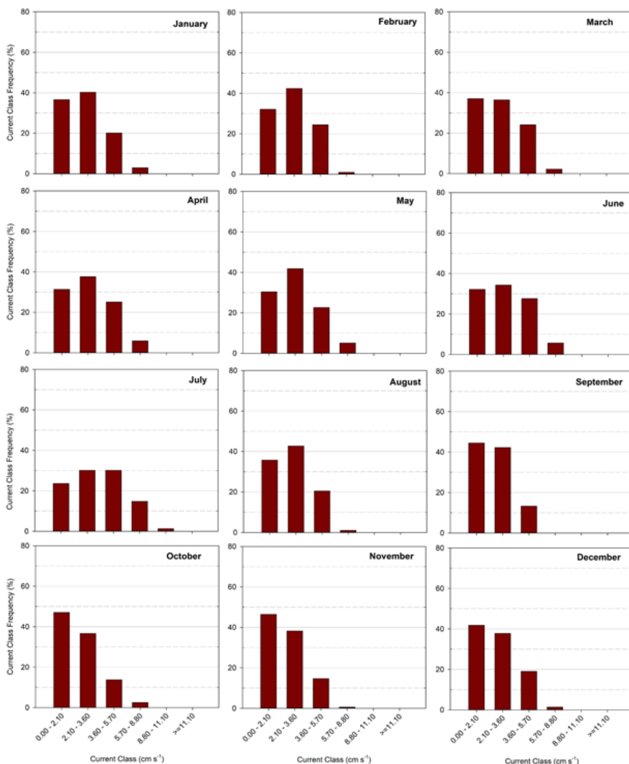
Figure 5-22. Average frequency (%) by current speed class (cm s -1 ) recorded from bin #4 of the upward-looking acoustic Doppler current profiler (ADCP) (300 kHz) on the Long Mooring between 15 October 2019 and 2 June 2021.
