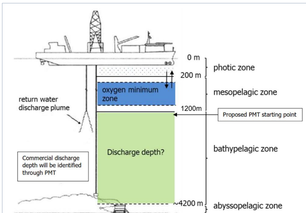
Figure 3-14. Proposed discharge depth for integrated system tests.
