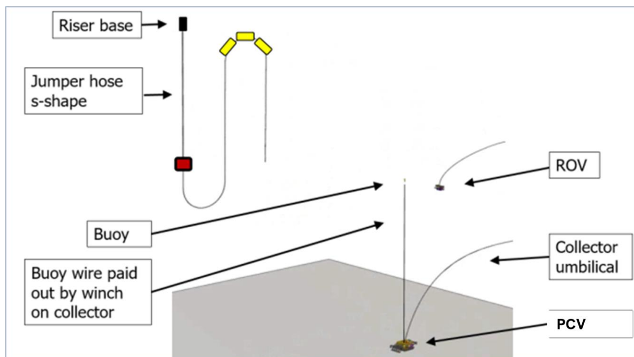
Figure 3-25. Connection configuration
