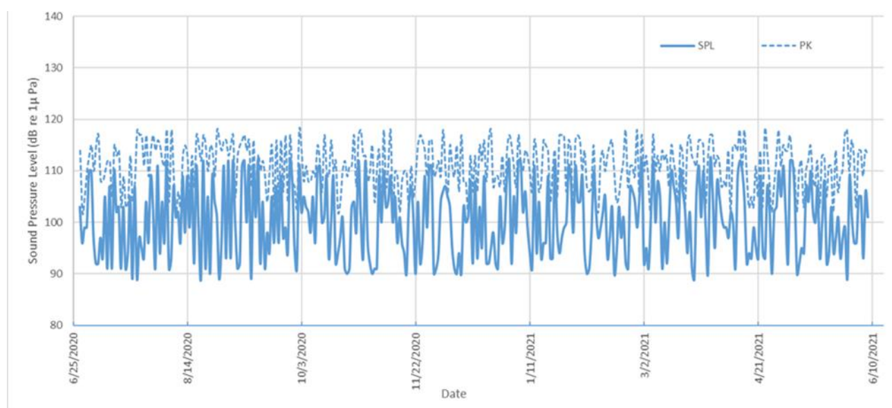
Figure 5-5. Daily averaged broadband root-mean-square sound pressure level (SPL) and zero-to-peak sound pressure level (PK) for the deep static acoustic recorder.
