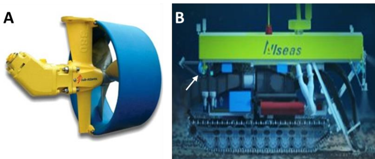
Figure 3-18. Thruster unit (A) and position on the PCV (B - dotted red circles)
