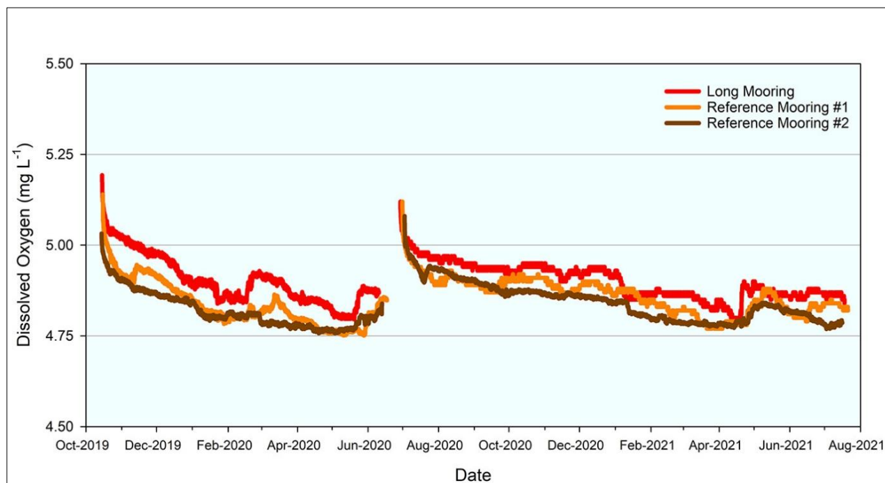
Figure 5-17. Running average of dissolved oxygen concentration values (mg L -1 ) by month at the proposed discharge water depth (~2,000 m) at the Long Mooring Site in the NORI-D block from October 2019 through July 2021.
