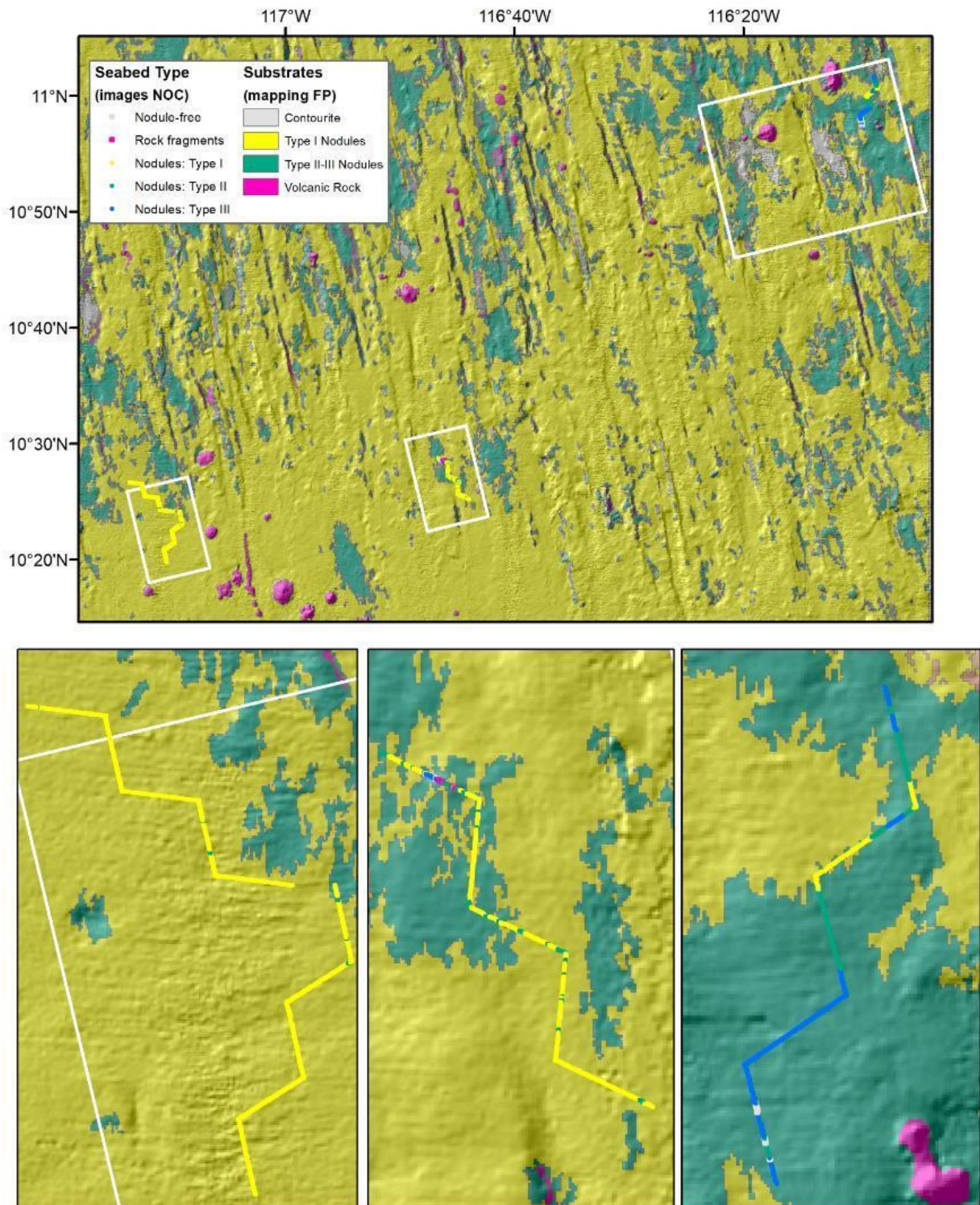
Figure 5-74. Comparison between predicted distribution of different seabed typologies (background, Fathom Pacific 2020) and observations obtained from in image data (lines, ROV surveys 2020)
