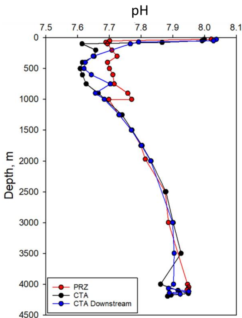
Figure 5-44. Plot of mean pH with depth for three sites sampled during Campaign 5B
