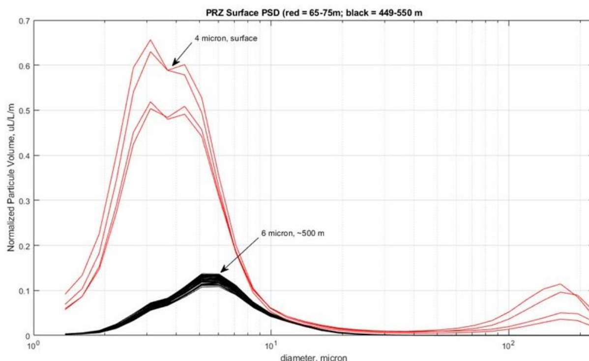
Figure 5-41. Particle size distribution in surface (65-75 m, red) and deeper (449-550 m, black) waters.
