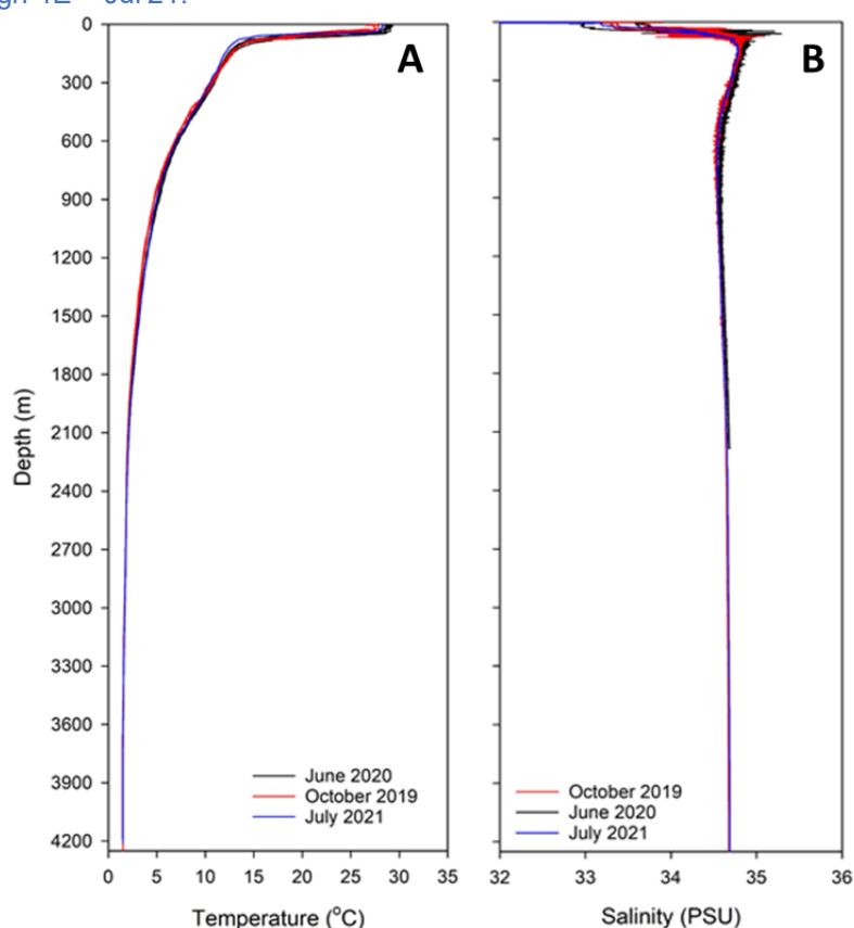
Figure 5-31. Average temperature and salinity profiles among Campaign 4A – Oct'19, Campaign 4D – Jun'20, and Campaign 4E – Jul'21.
