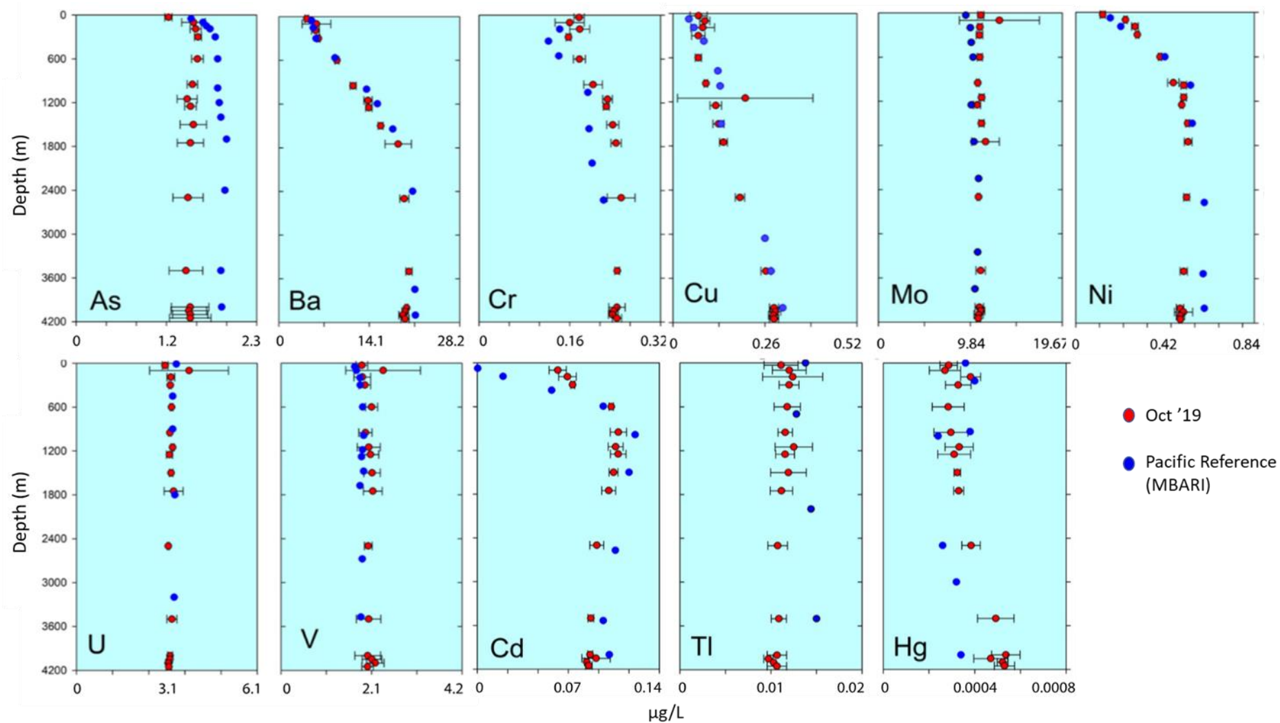
Figure 5-46. Concentrations of metals and metalloids from seawater samples collected on Campaign 4A (note: not GEOTRACES compliant)
