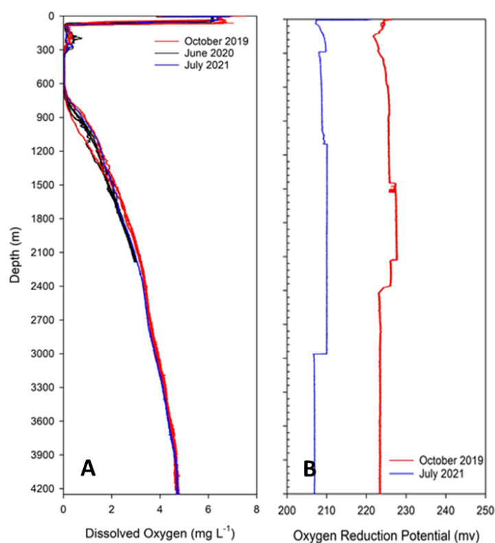
Figure 5-32. Average dissolved oxygen profiles among Campaign 4A – Oct'19, Campaign 4D – Jun'20, and Campaign 4E – Jul'21. Average oxygen reduction profiles among Campaign 4A – Oct'19 and Campaign 4E – Jul'21
