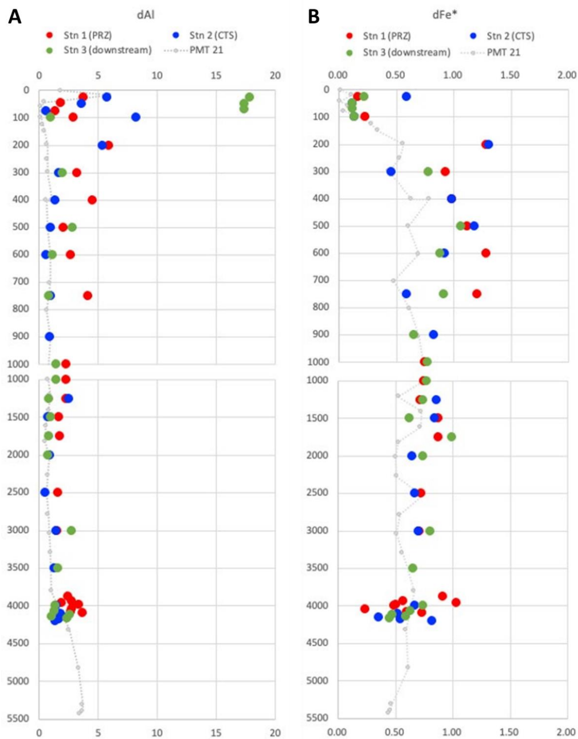
Figure 5-49. Vertical profiles for FIA-based dissolved Al and Fe during Campaign 5B. PRZ (red circle), CTS (blue circle), and downstream (green circle) were shown together with previous GEOTRACES GP15 station (samples were collected at 11°N, 152°W on 2018 November 1 st during the GP15-PMT cruise). These data are unpublished and should be considered preliminary.
