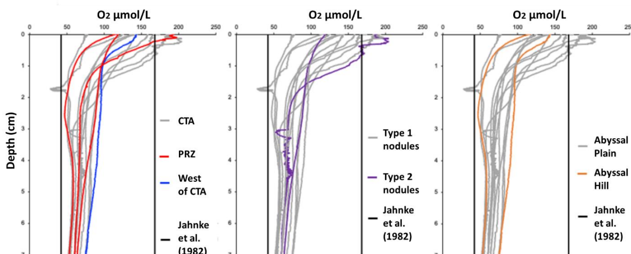
Figure 5-56. Ex-situ oxygen profiles colour coded for sample region, nodule type and geofrom (left to right).
