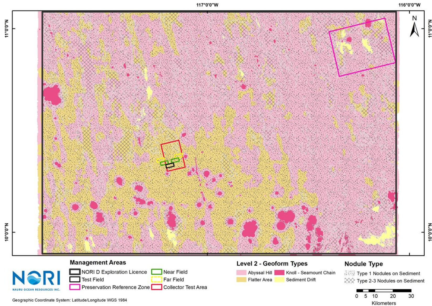
Figure 5-71. NORI-D Level 2 geoforms and Level 2 substrates
