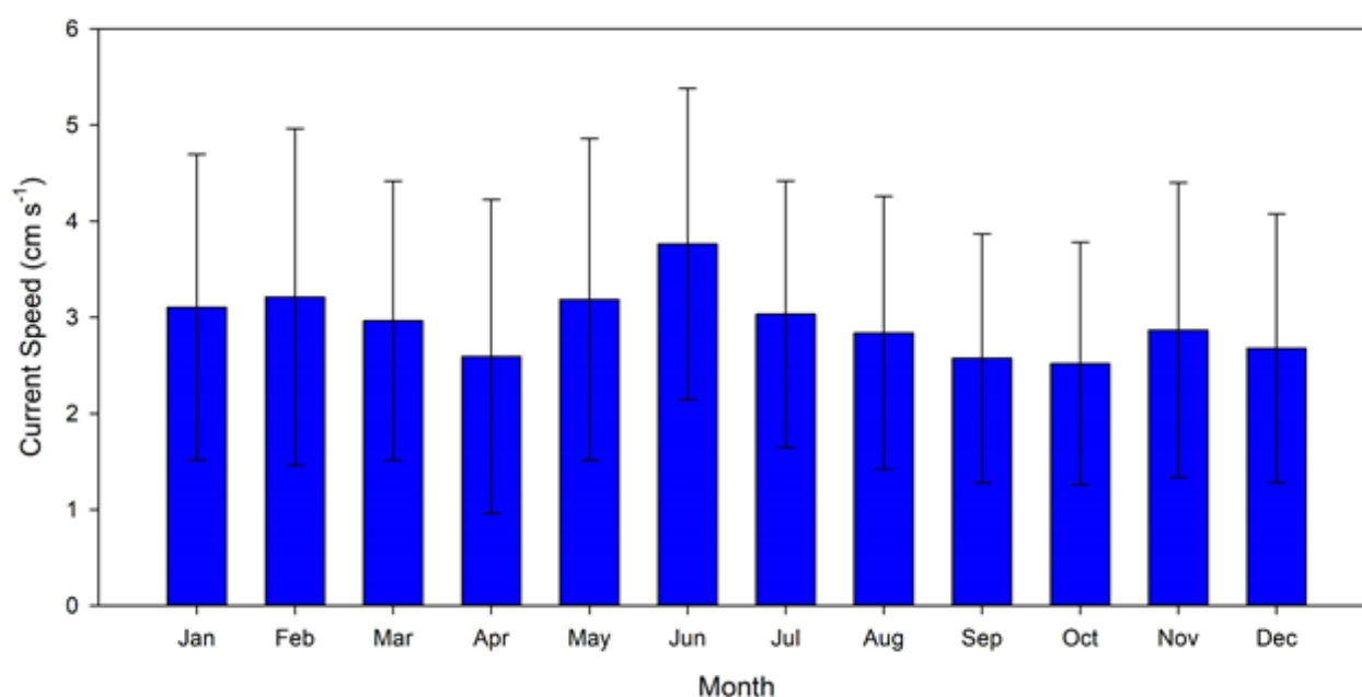
Figure 5-25. Average ( \pm standard deviation) current speeds (cm s -1 ) recorded from bin #4 of the downward-looking acoustic Doppler current profiler (ADCP) (600 kHz) at 4,321 m water depth (i.e., 5 m above the seafloor) on the Long Mooring between 15 October 2019 and 24 April 2021.
