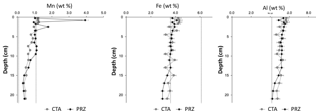
Figure 5-61. Preliminary data of on-going total metal analysis.
