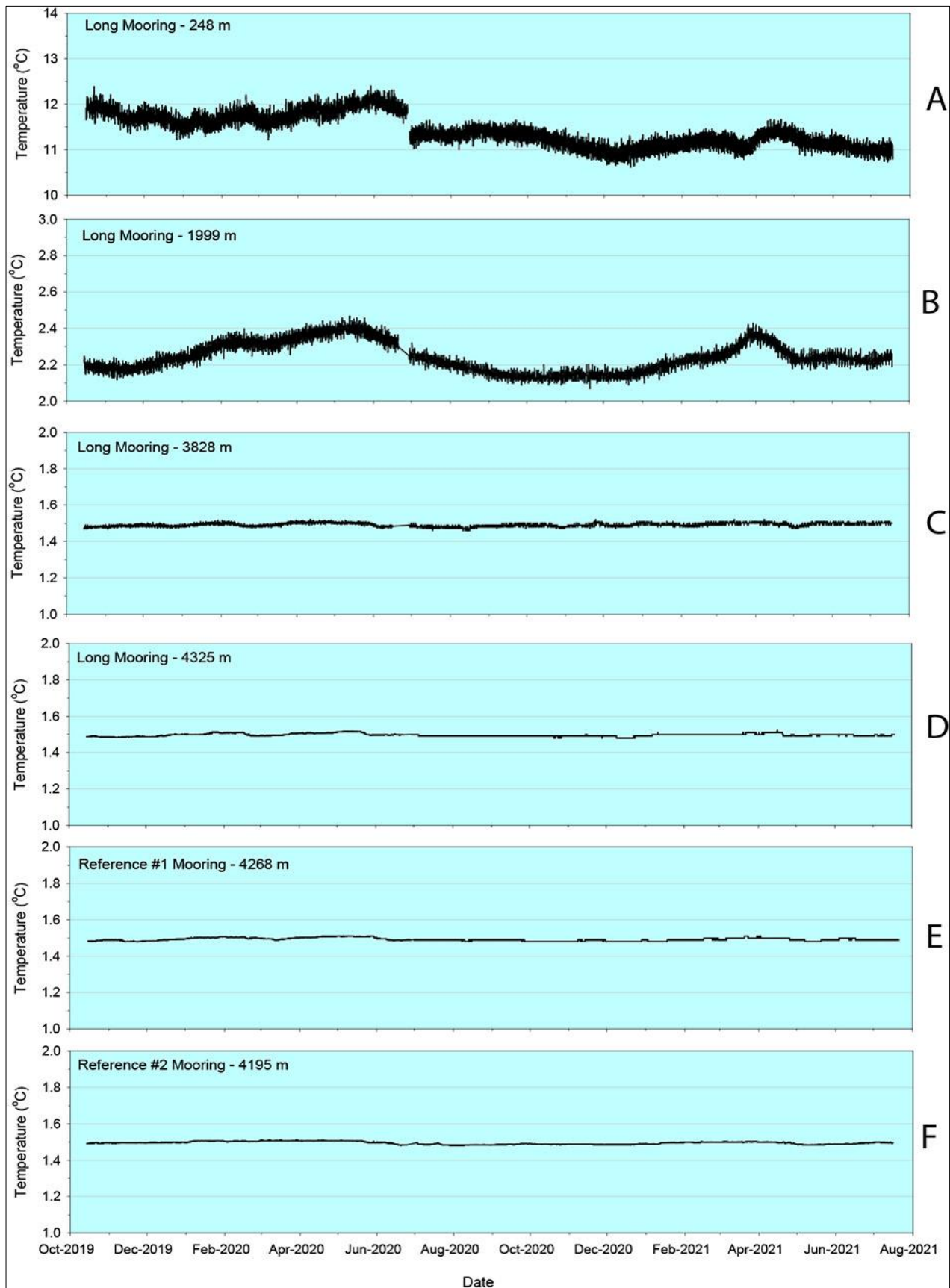
Figure 5-11. Near-continuous temperatures values (°C) at selected Long (A to D) and Reference (E to F) mooring conductivity-temperature-depth (CTD) instrumentation depths in the NORI-D block from October 2019 through July 2021. Note the difference in y-axis scales.
