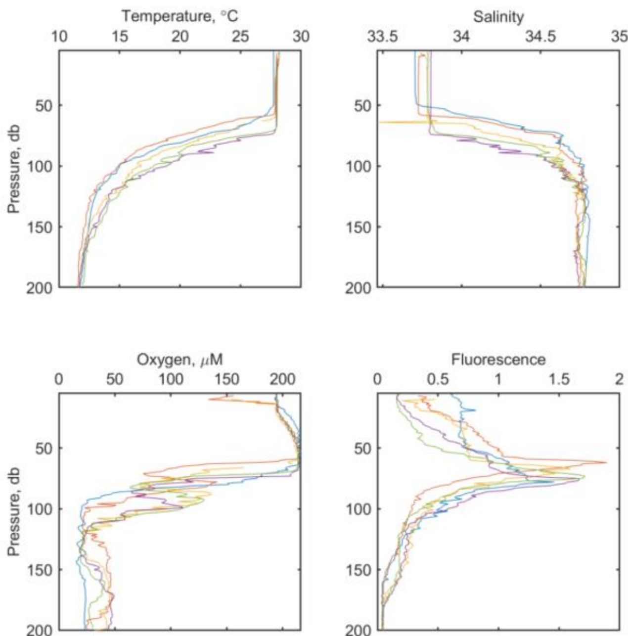
Figure 5-40. Vertical profiles of temperature, salinity, dissolved oxygen, and fluorescence in the upper 200 m of the water column at the CTA site during Campaign 5B.
