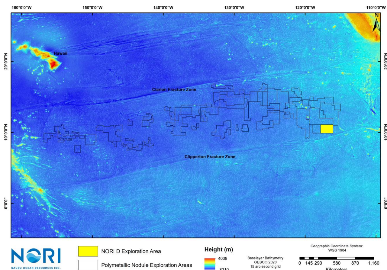
Figure 5-64. Bathymetric overview of the CCZ
