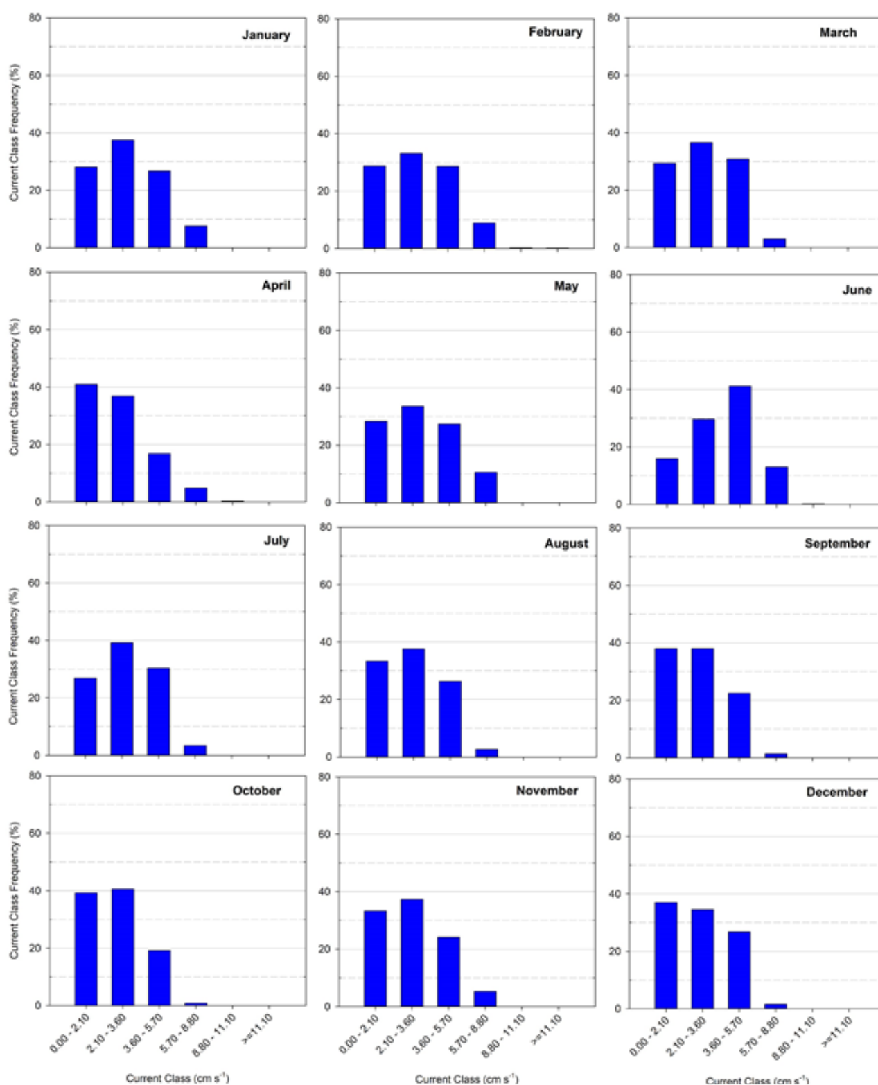
Figure 5-26. Average frequency (%) by current speed class (cm s -1 ) recorded from bin #4 of the downward-looking acoustic Doppler current profiler (ADCP) (600 kHz) at 4,321 m water depth (i.e., 5 m above the seafloor) on the Long Mooring between 15 October 2019 and 24 April 2021.
