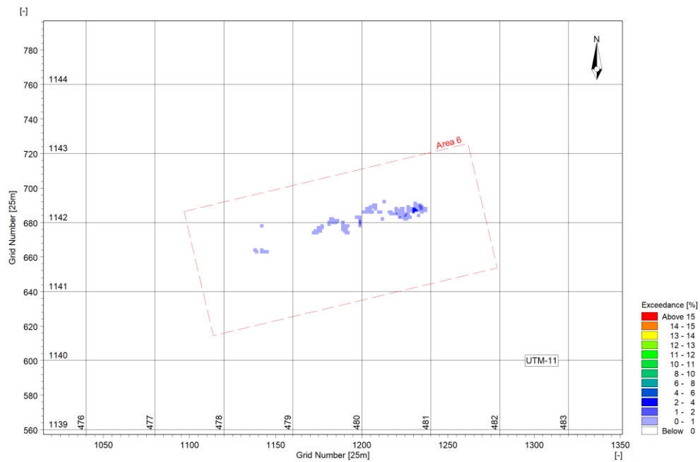
Figure 3.76 Scenario STR3a: Exceedance percentage of 10mg/l, from the start of production to 48 hours post-production at 5m above the seabed
